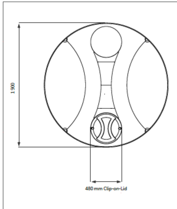
TOP VIEW
