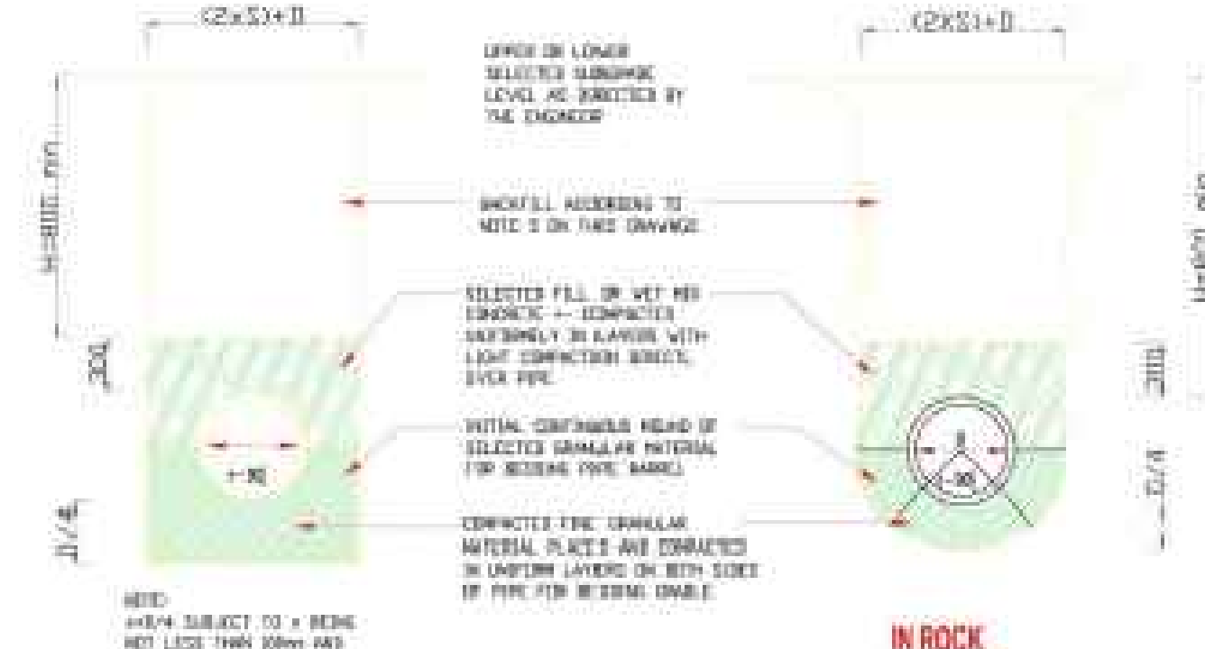
CLASS B BEDDING
