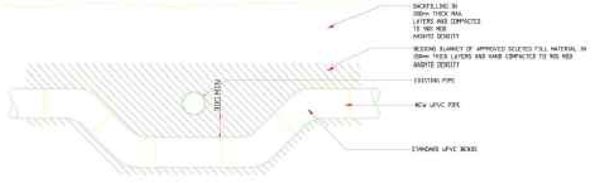
TYPICAL UNDERGROUND PIPE CROSSING DETAILS IF ON SAME LEVEL OPTION 1
