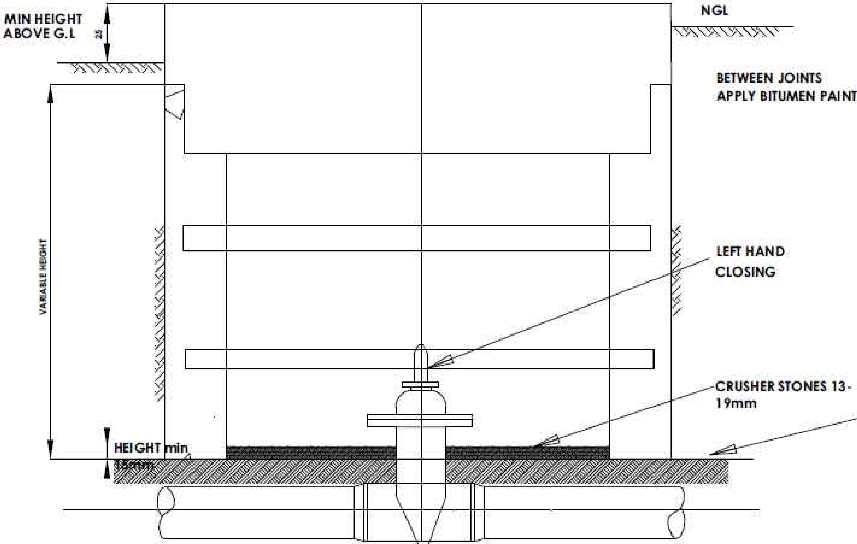
SECTION DETAIL OF VALVE BOX FOR PIPES
