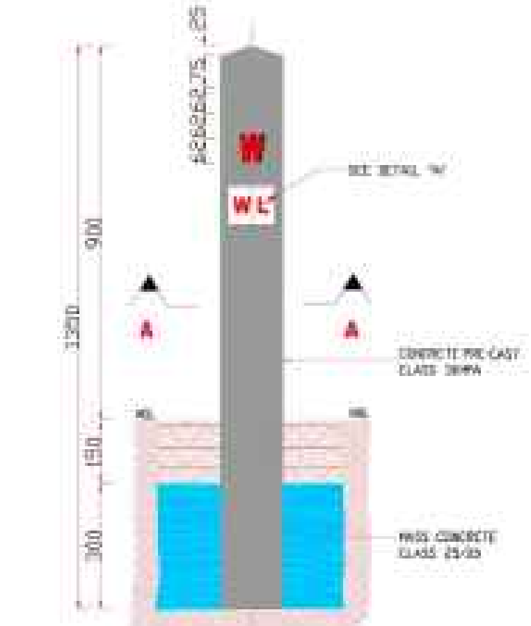
PIPELINE PRECAST CONCRETE MARKER POST
