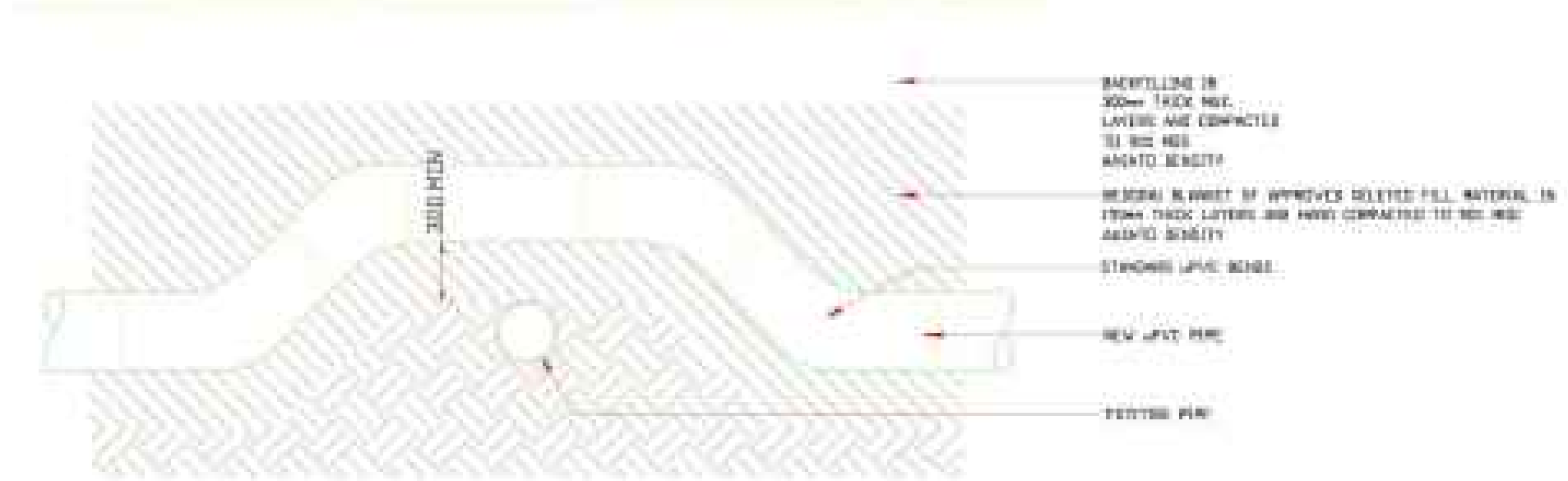
TYPICAL UNDERGROUND PIPE CROSSING DETAILS IF ON SAME LEVEL OPTION 2
