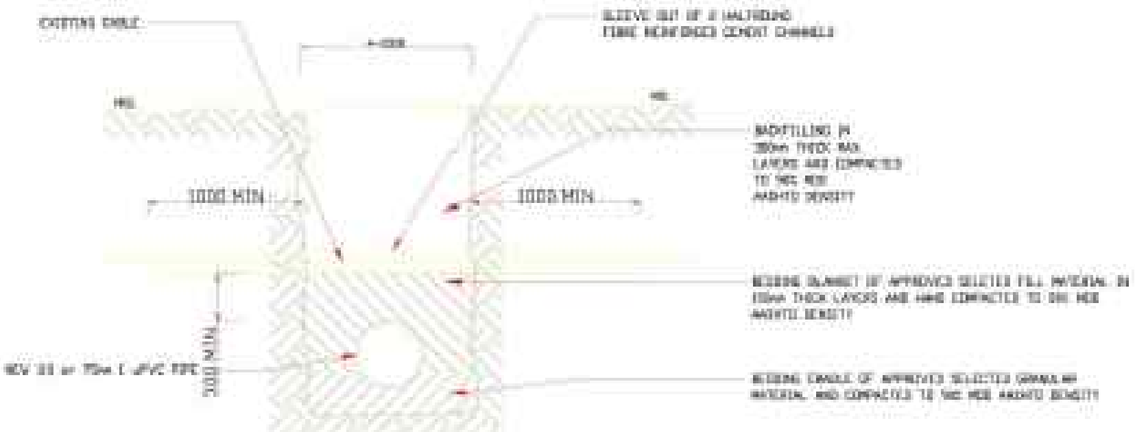
TYPICAL UNDERGROUND CABLE CROSSING DETAIL 1:30
