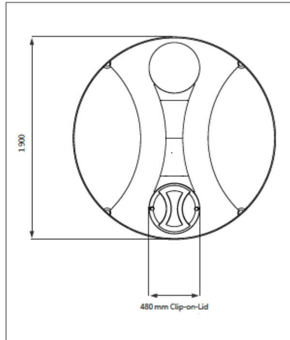
TOP VIEW
