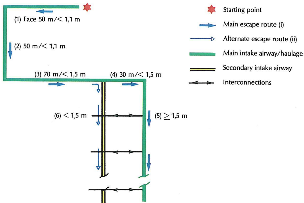
Plan view of escape route
