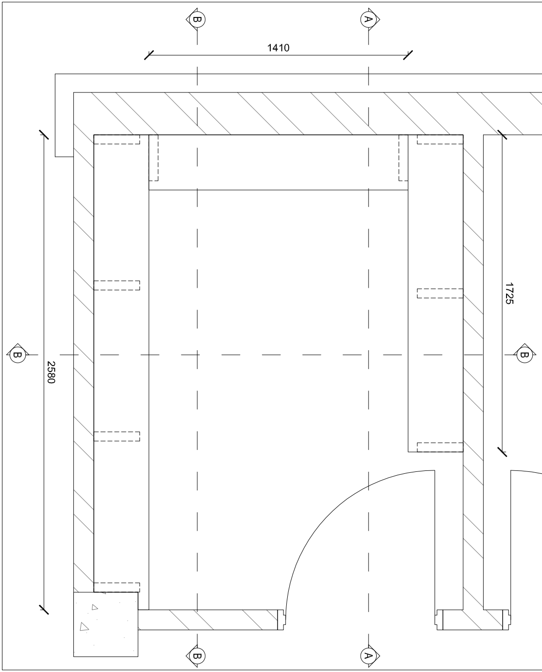
TYPICAL CLEANERS STORE SHELVING LAYOUT SCALE 1:20
