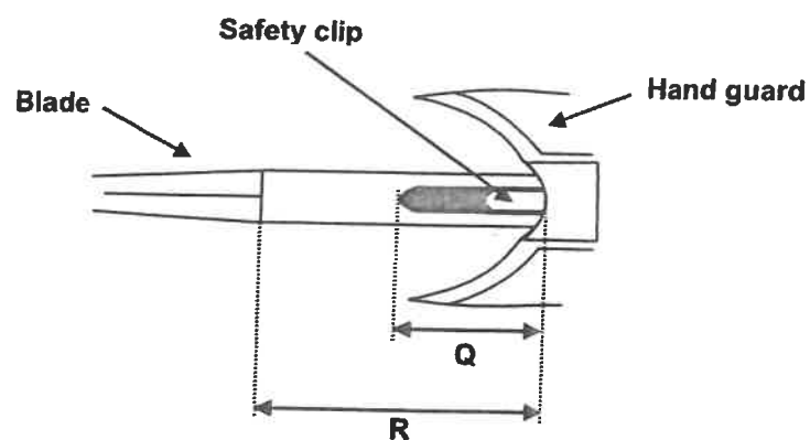
Figure 2(b) - Dimensions of dagger
