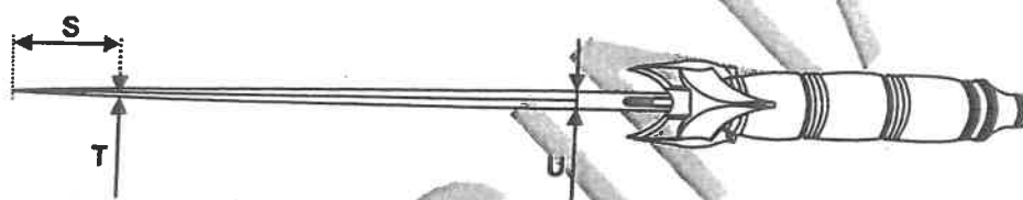
Figure 2(c) - Dimensions of dagger
