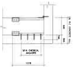
TYPE 'A' LADDER LAYOUT PLAN (1:10, SEE ALSO)
