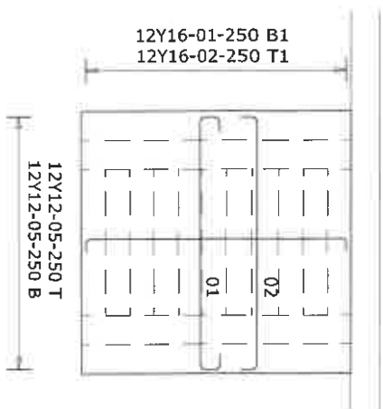
R.C. STAIR LAYOUT PLAN
