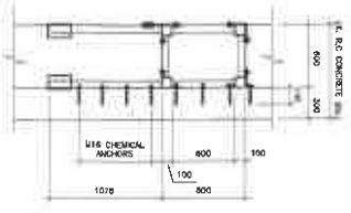
TYPE 'B' LADDER LAYOUT PLAN (1:10, SEE ALSO)
