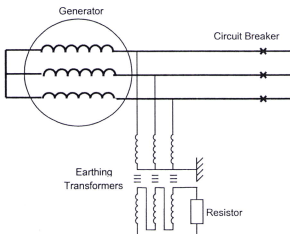
Figure 4: Generator Earthing
