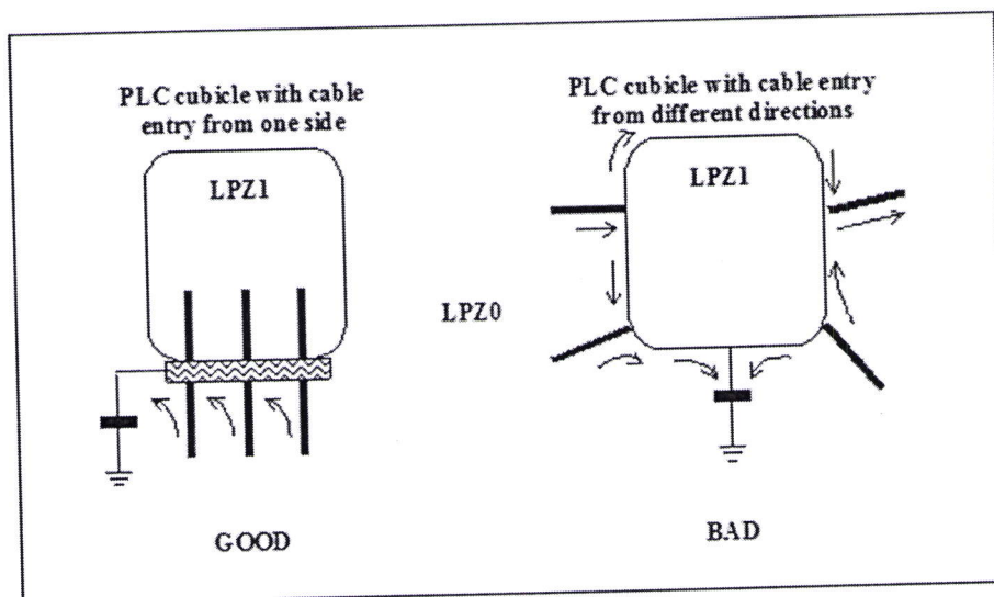
Figure 3: Minimizing of surface current by single entry point of cables
