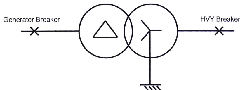
Figure 5: Generator Transformer Earthing
