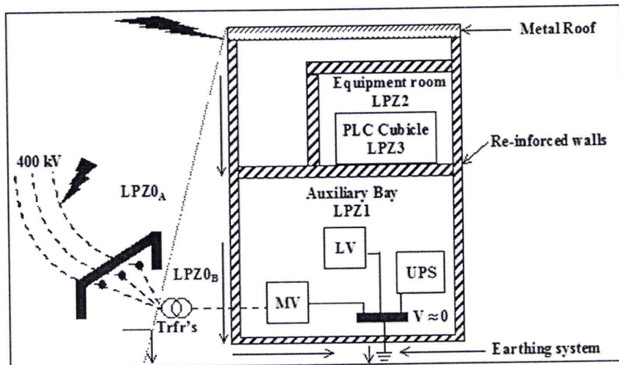
Figure 1: Power Station typical Zone Definition
