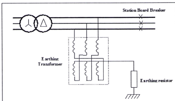
Figure 7: Station Transformer earthing arrangement
