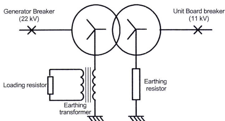
Figure 6: Unit transformer earthing
