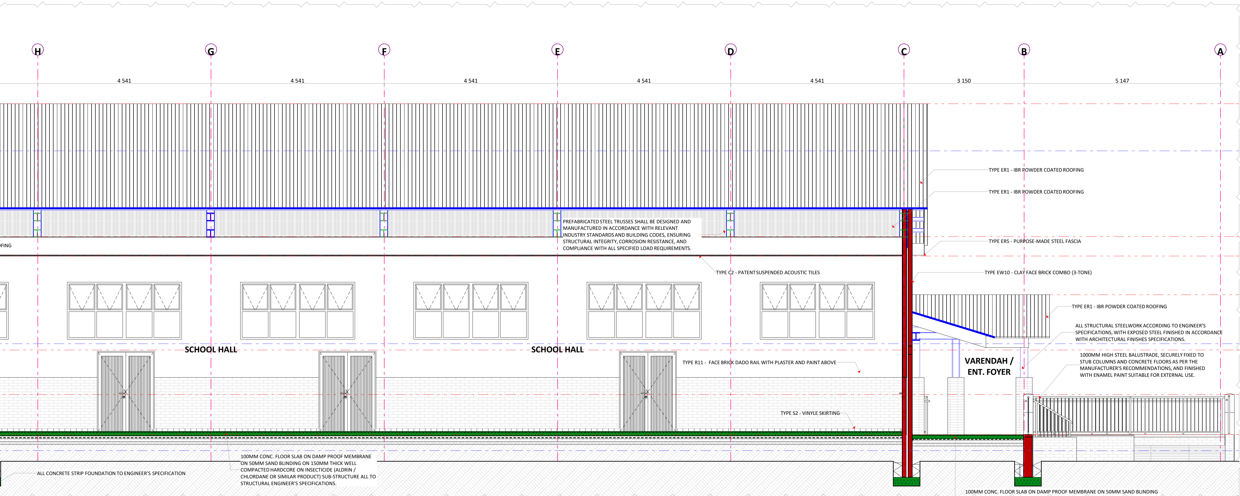
SECTION - S-44 PART B 1:50
