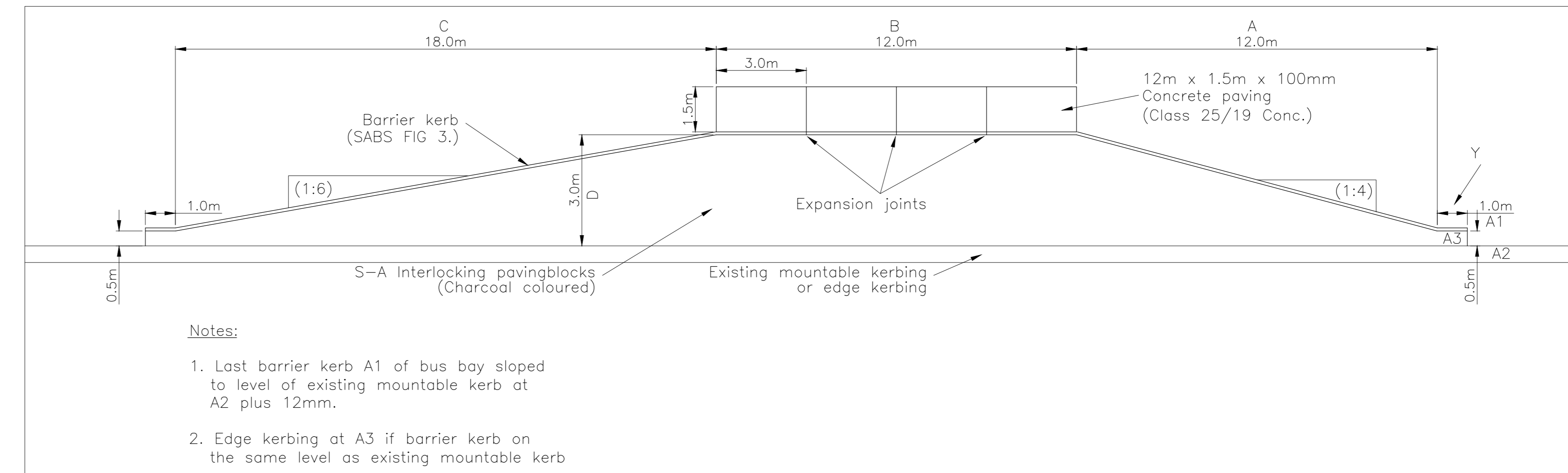
LAYOUT PLAN OF TYPICAL BUS BAY SCALE - 1: 150
