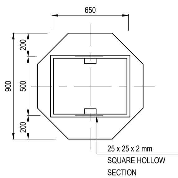
SINGLE SUPPORT REINFORCEMENT FOR STOP SIGNS
