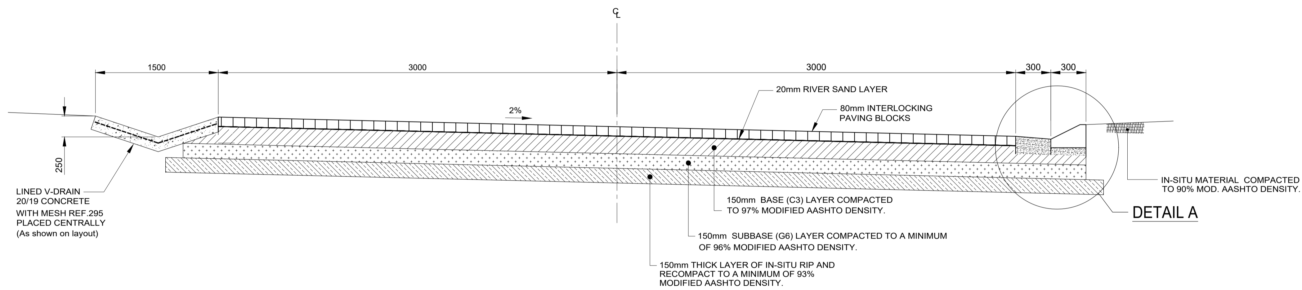
TYPICAL CROSS-SECTION & PAVEMENT DESIGN DETAILS
