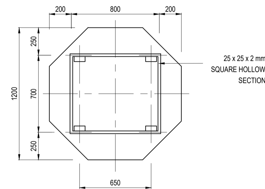
DOUBLE SUPPORT
