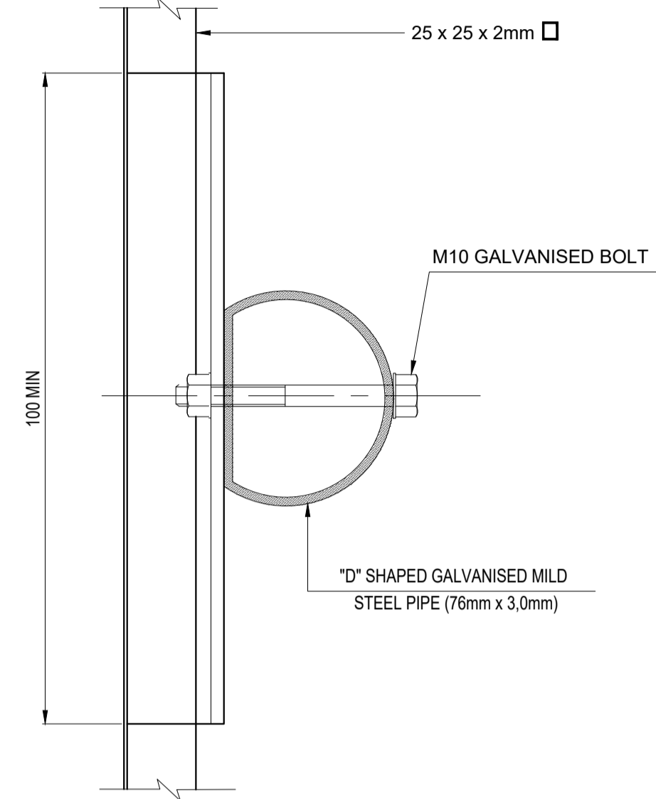
SIDE ELEVATION
