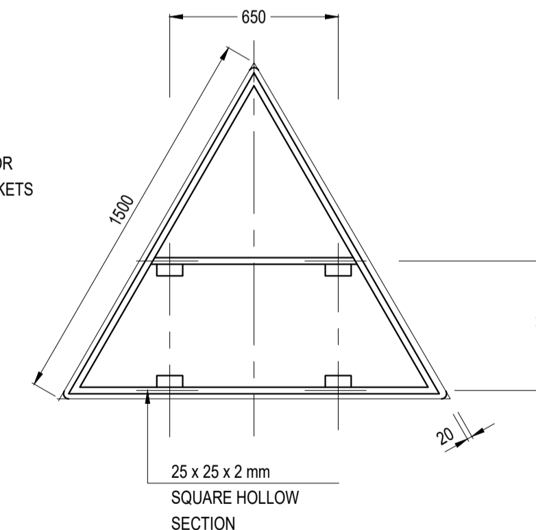
DOUBLE SUPPORT
