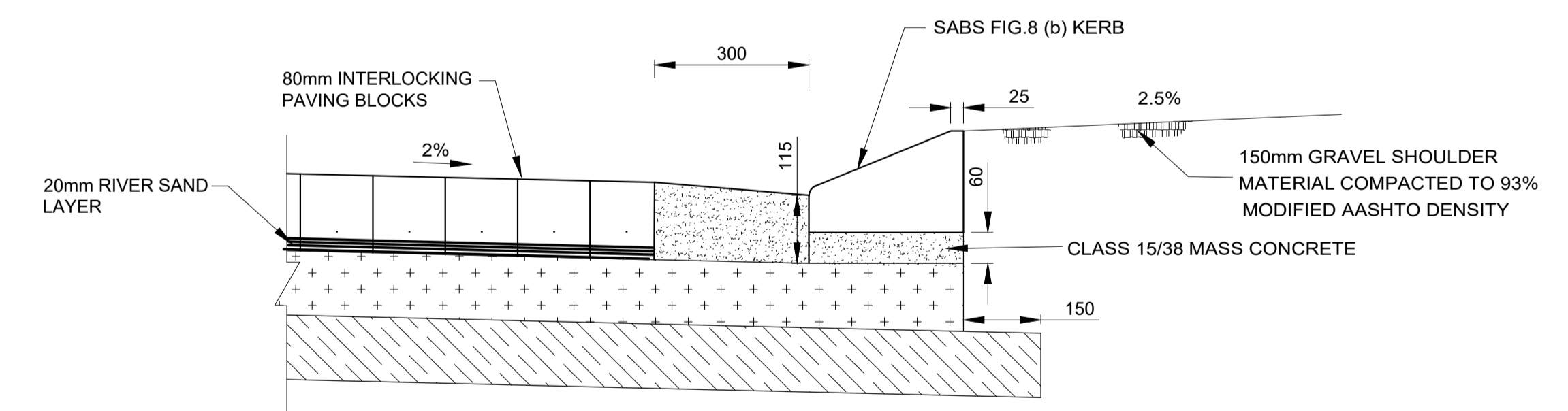
DETAIL A
