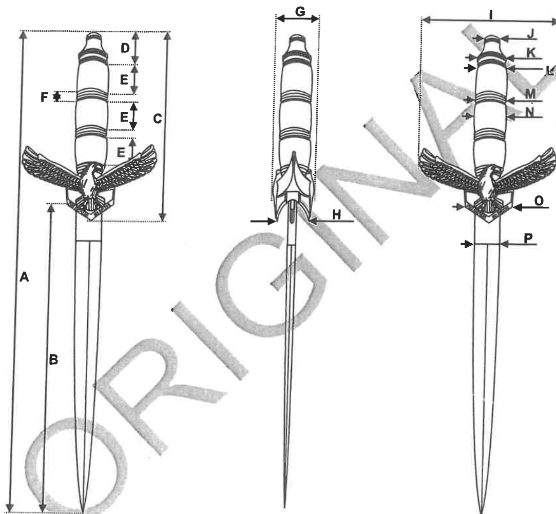
Figure 2(a) - Dimensions of dagger
