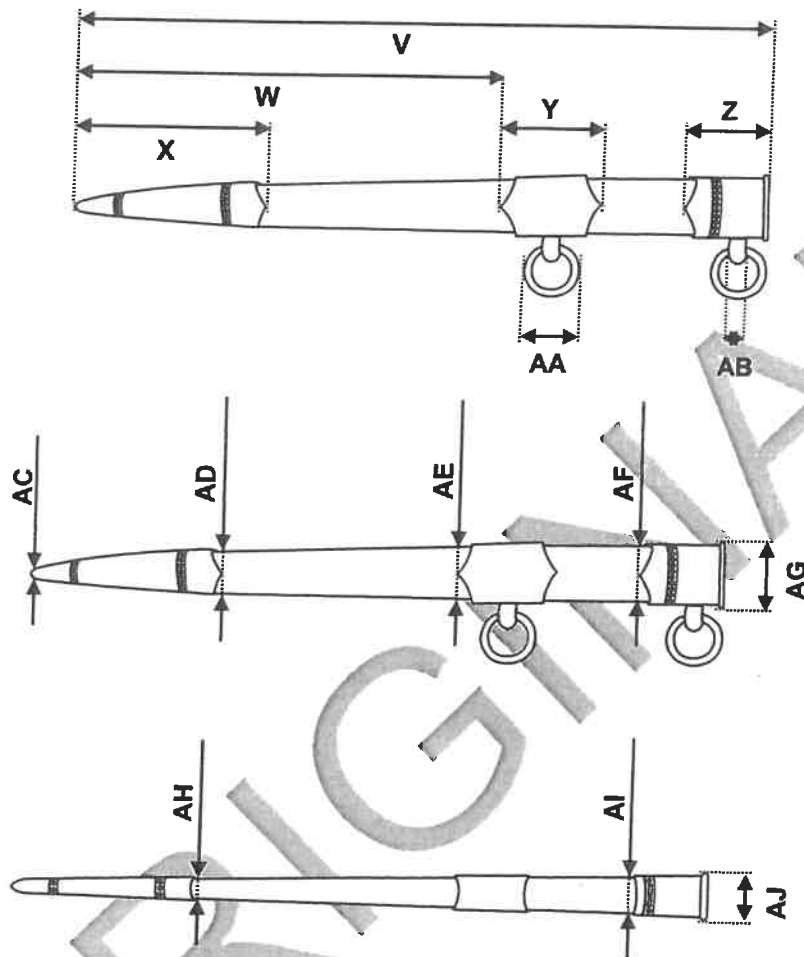
Figure 3 – Dimensions of scabbard
