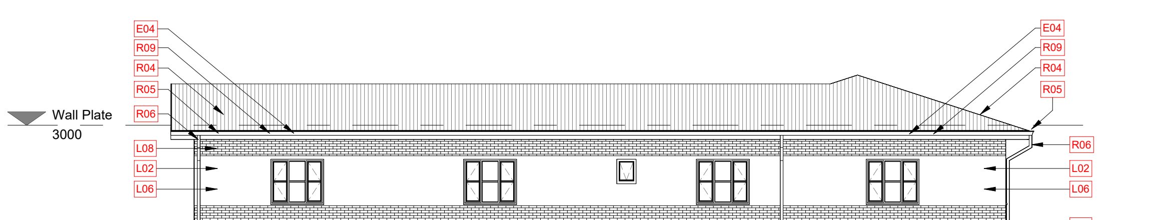
North West 1 : 100
