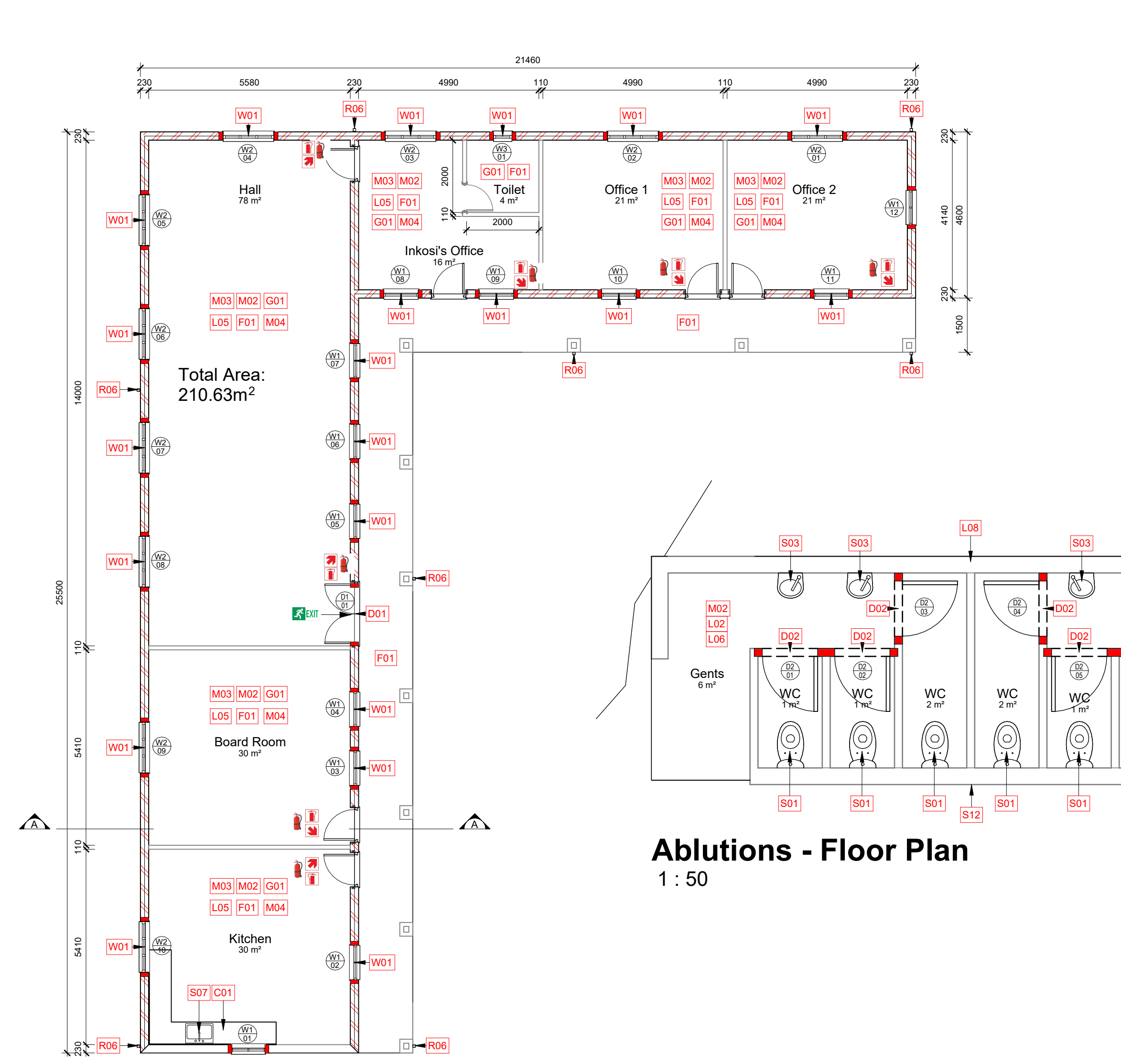
Main Building - Floor Plan
