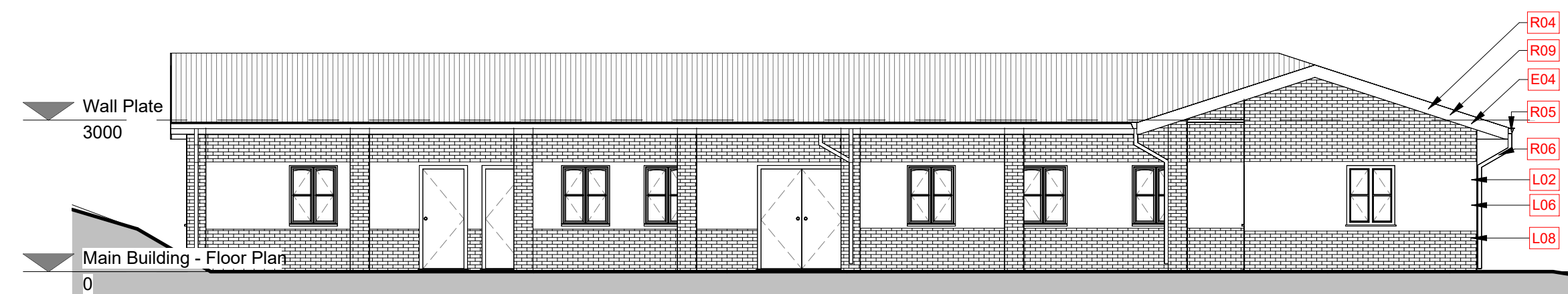
North East 1 : 100
