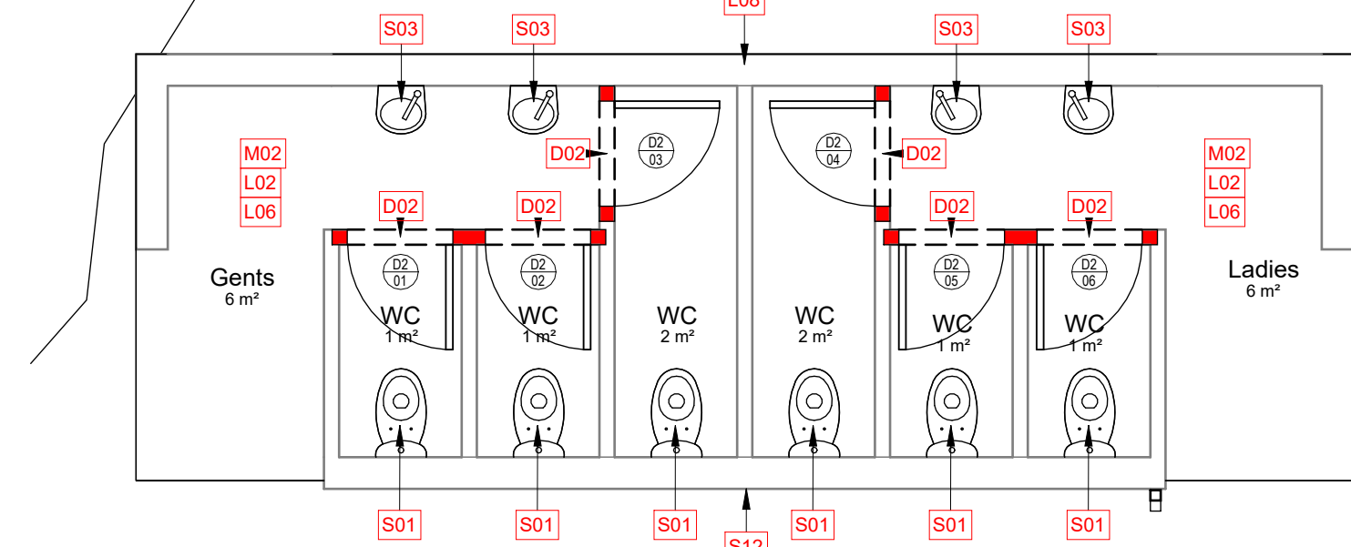
Ablutions - Floor Plan
