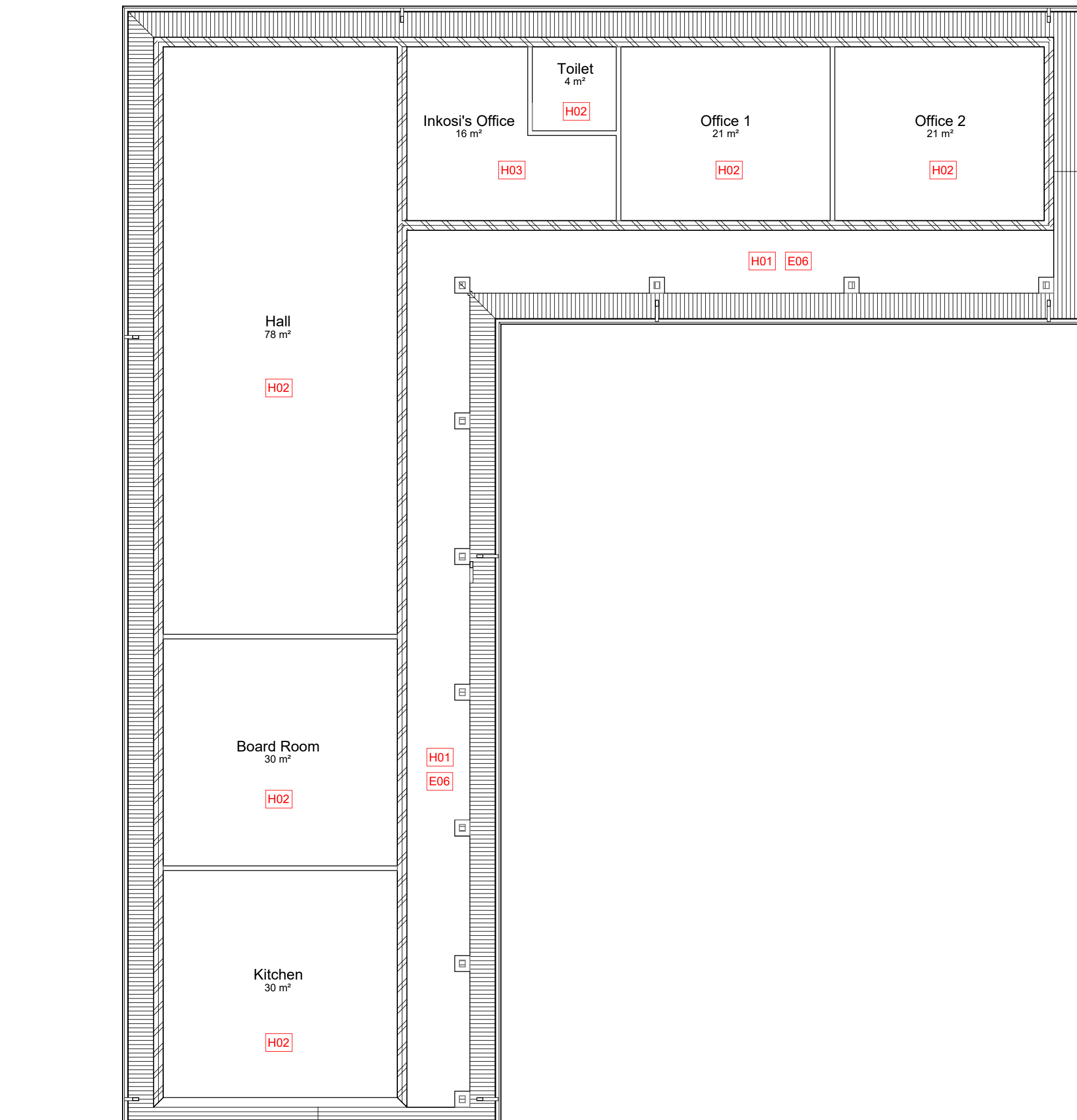
Main Building - Ceiling Plan
