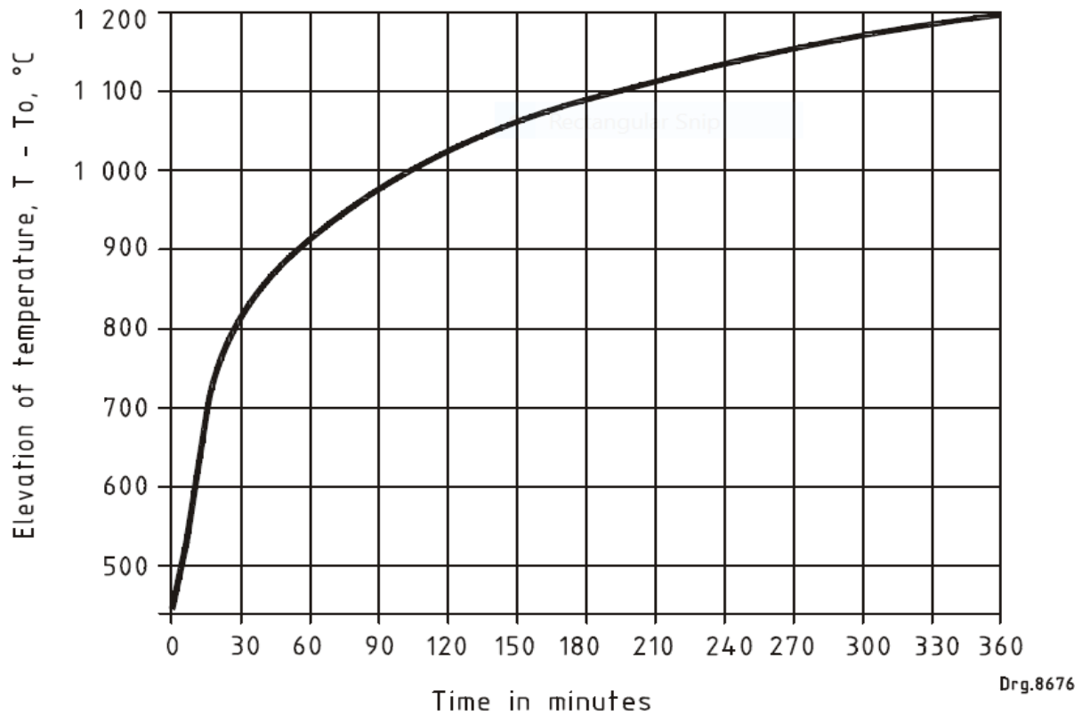
Figure 1 — Standard time-temperature curve
