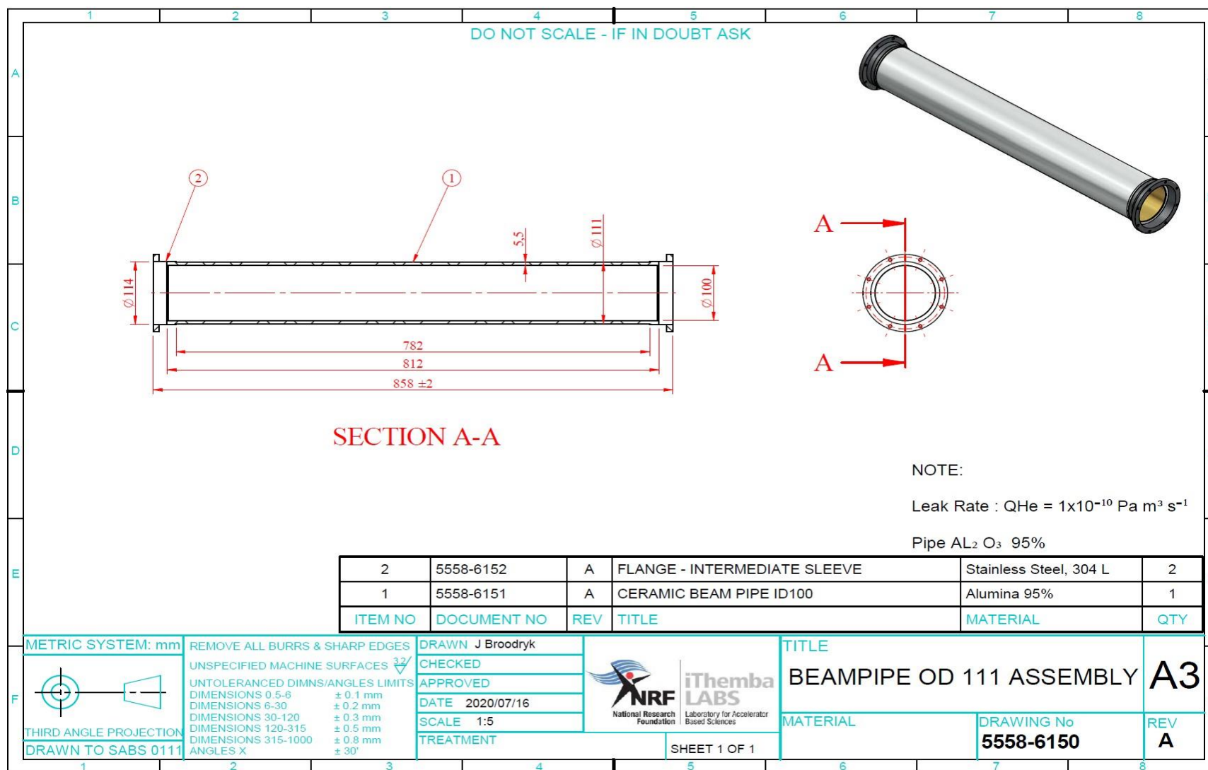
Figure 3: Drawing of the ceramic beam pipe with flanges and the dimensions.
