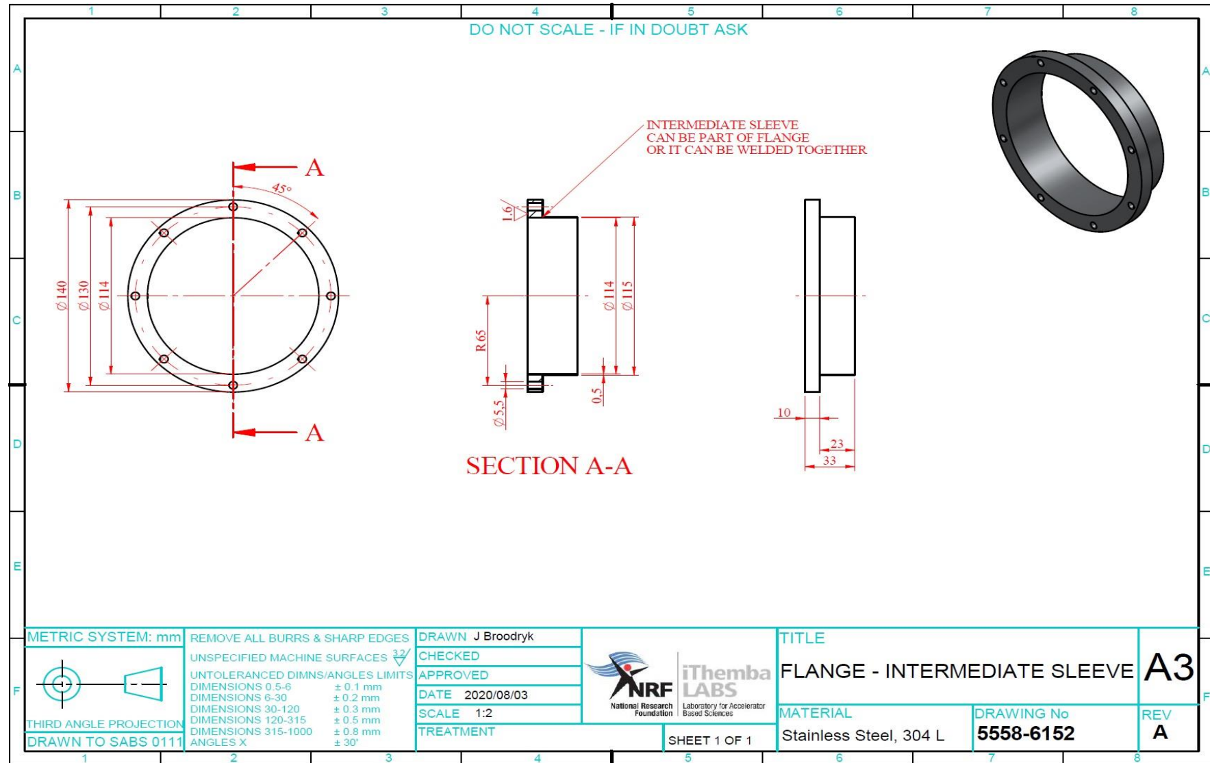
Figure 4: Drawing of the stainless steel flanges.
