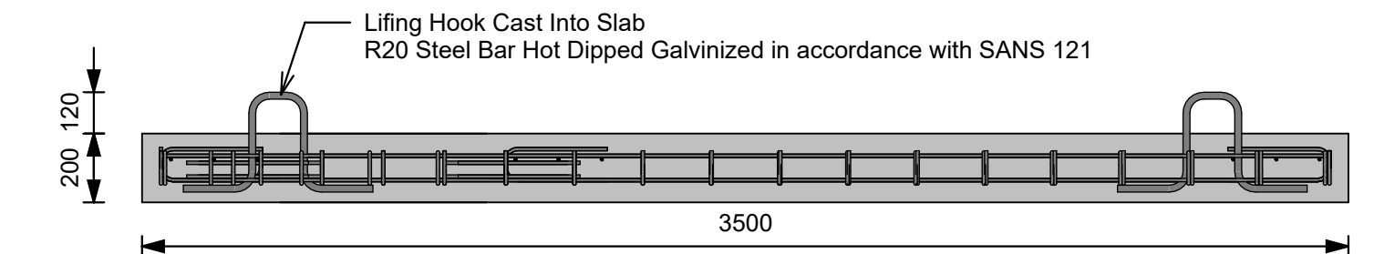
Section Through Manhole Cover Slab
