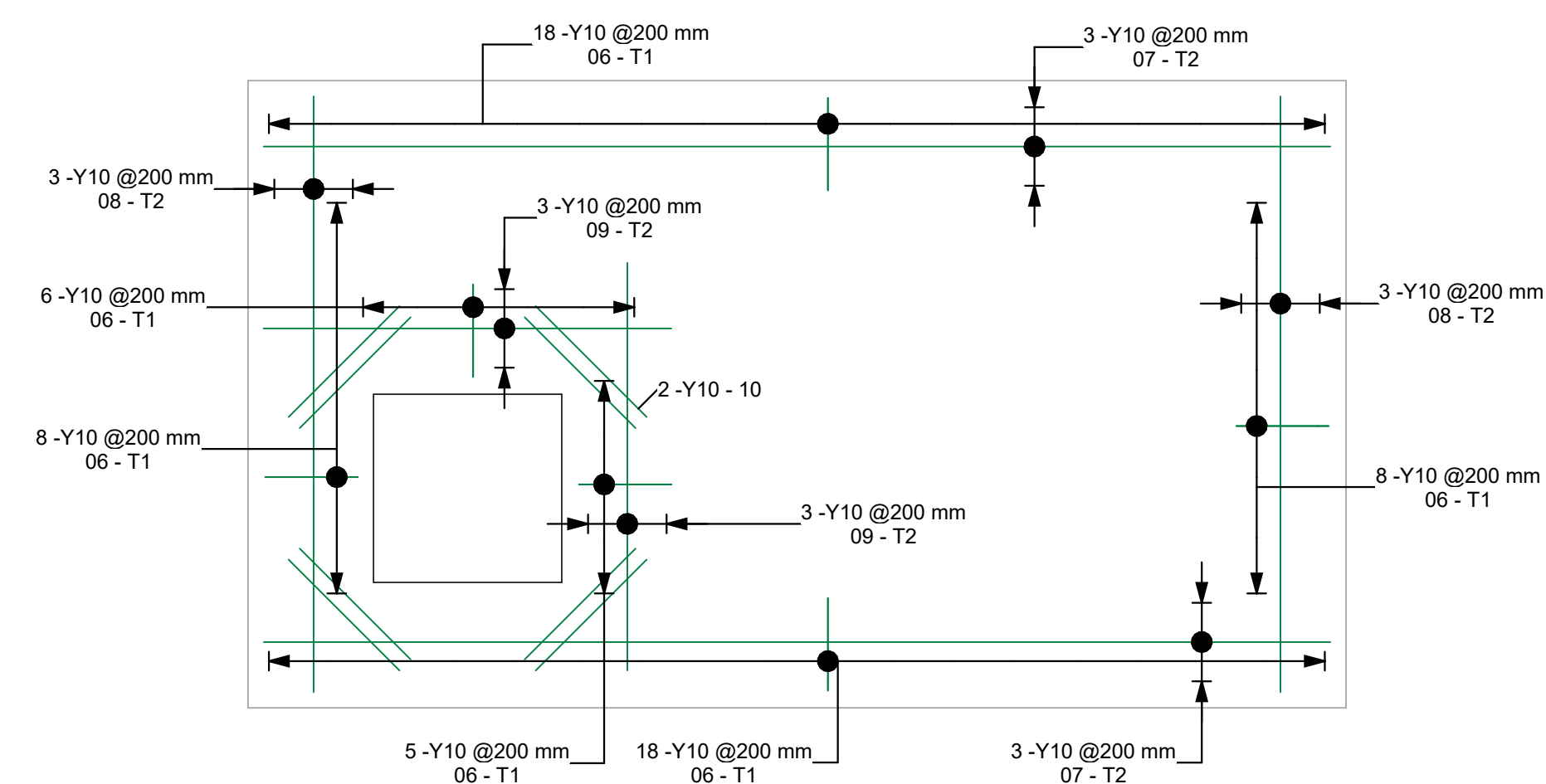
Top Reinforcement Details
