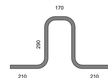
Lifting Hook Dimensions
