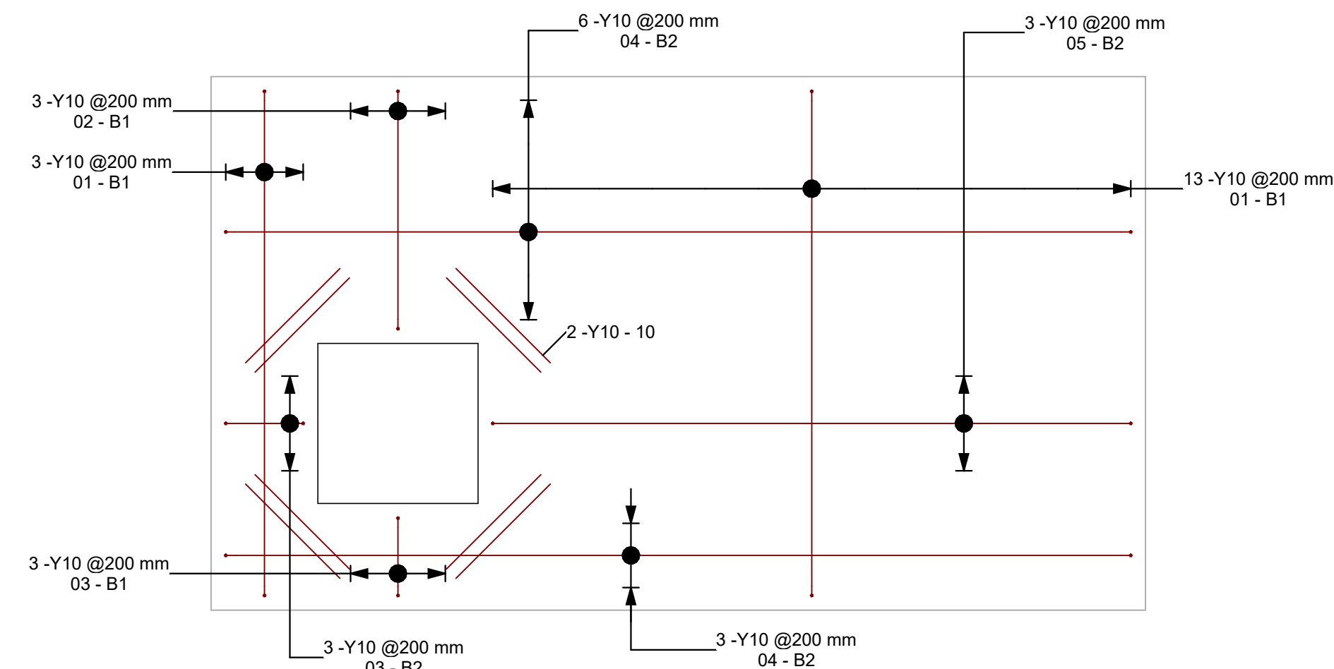
Bottom Reinforcement Details
