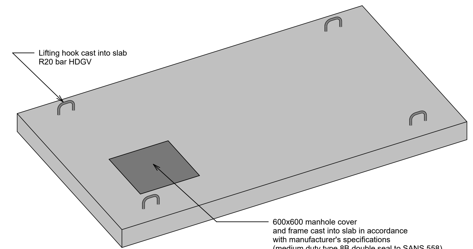
Manhole Cover Slab 3D View
