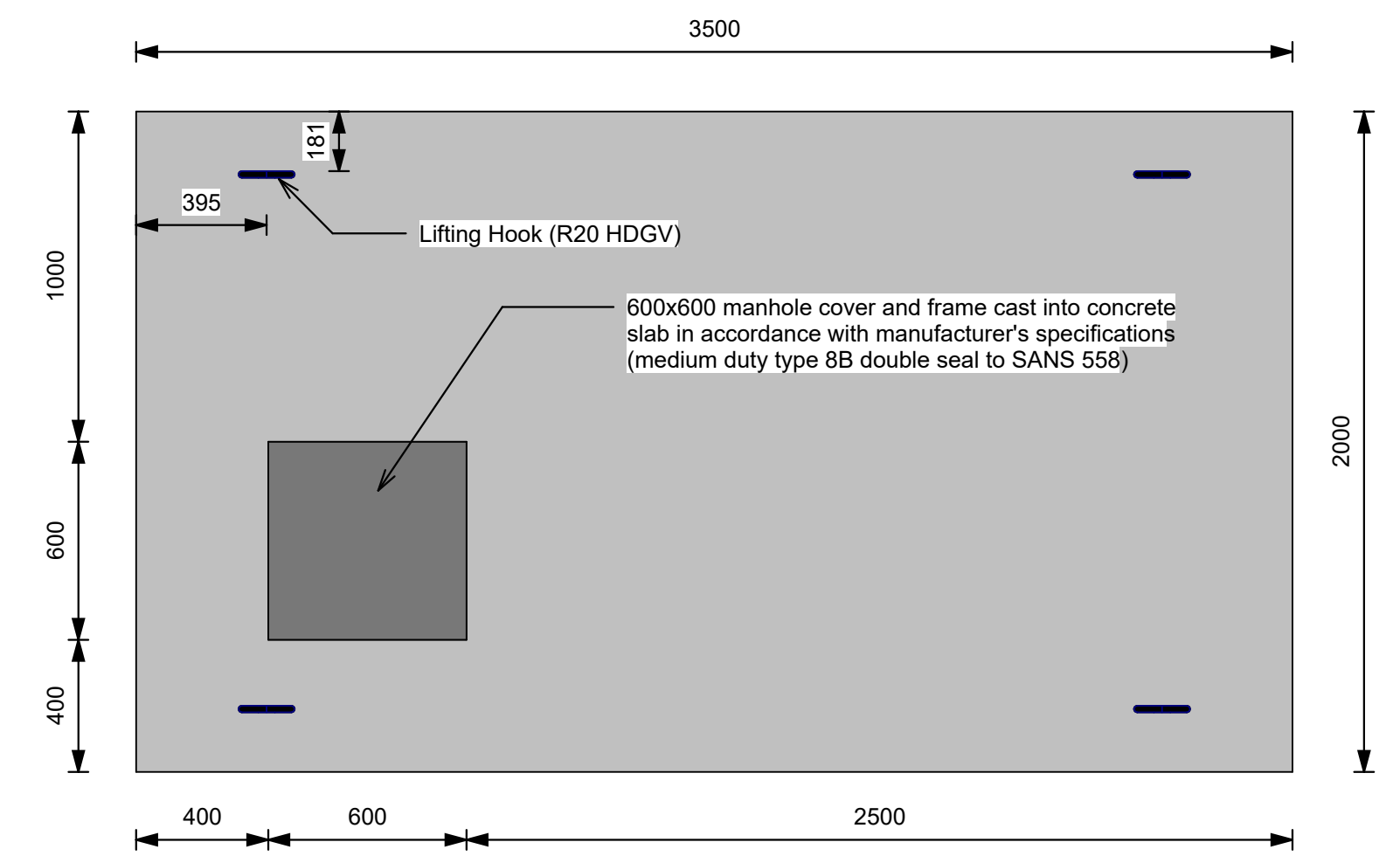
Plan View - Concrete Manhole Cover Slab
