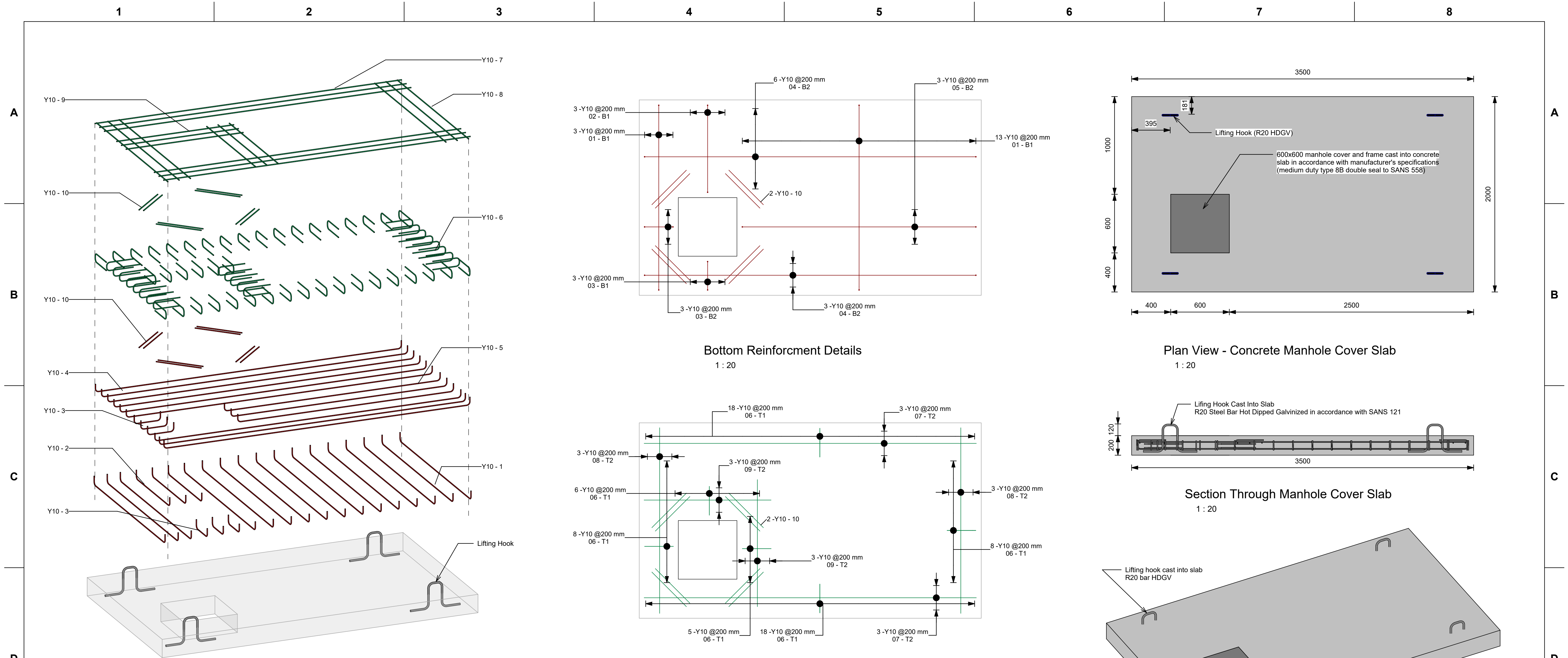
Top Reinforcement Details
