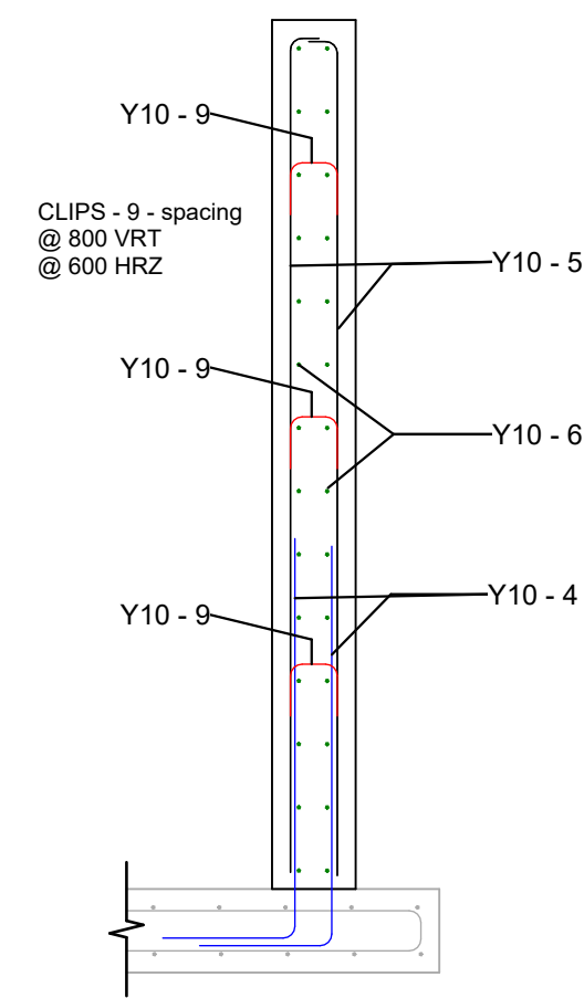
TYPICAL SECTION - WALL REINFORCEMENT 1 : 25
