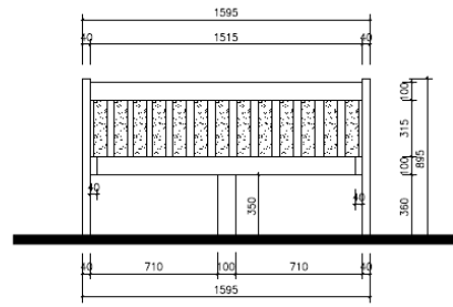
BACK VIEW SCALE 1:20
