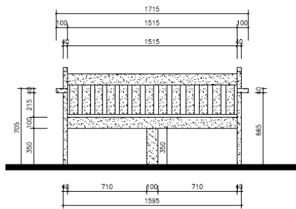
FRONT VIEW SCALE 1:20
