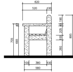
SIDE VIEW SCALE 1:20
