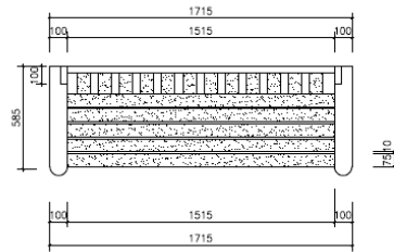
TOP VIEW SCALE 1:20
