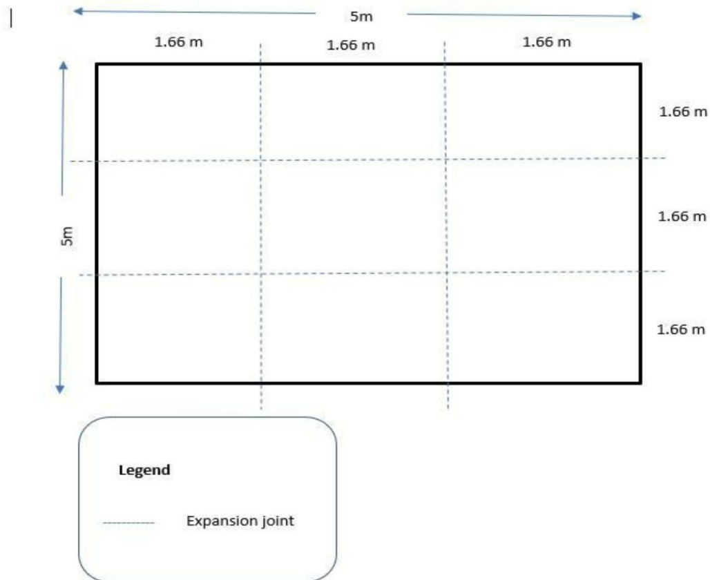
Figure #2: Dimensions of the plinth/slump (N.B expansion joints should be as shown in the diagram)
