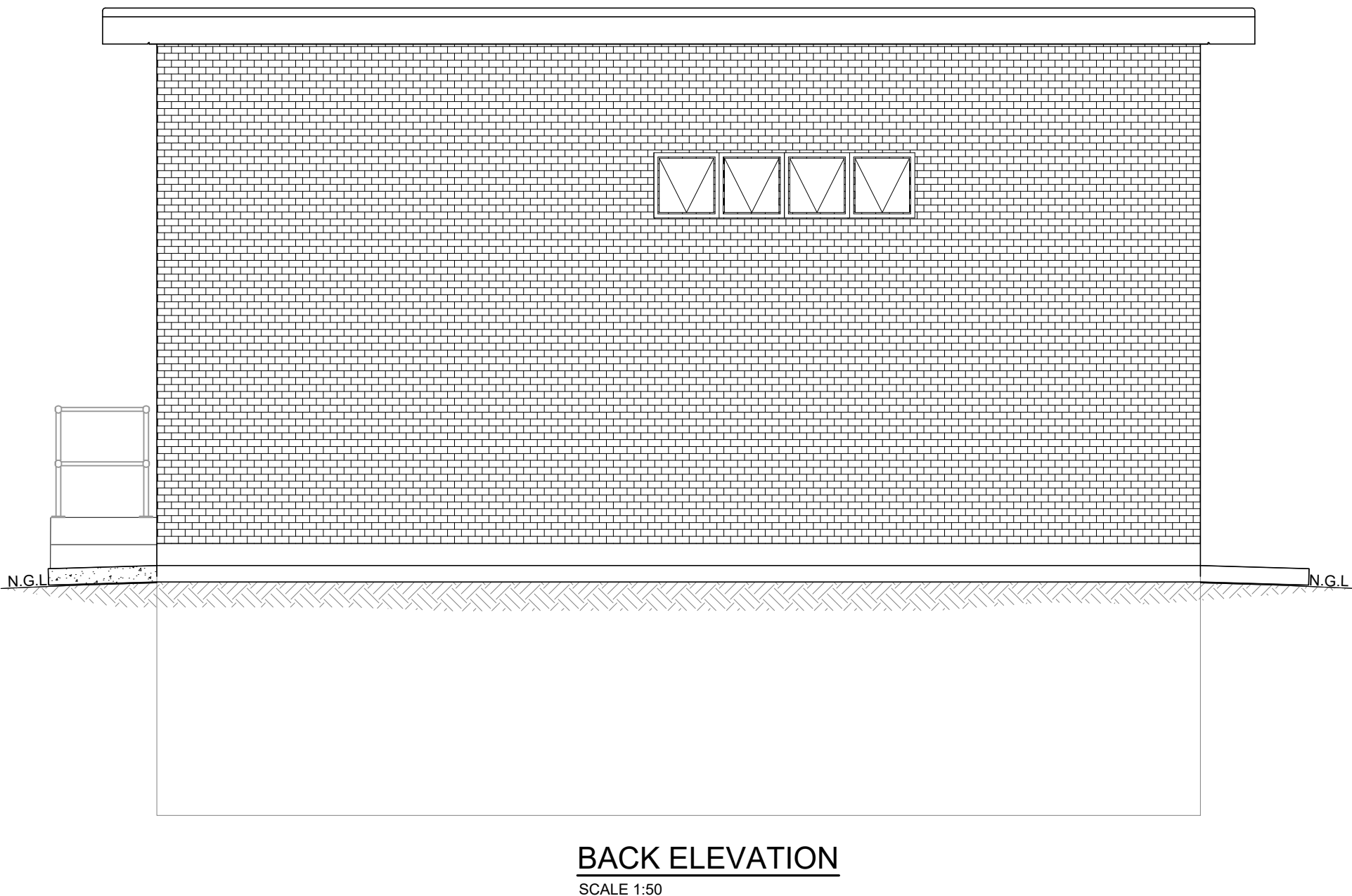
RAW WATER PUMP STATION ELEVATIONS SCALE 1:50
