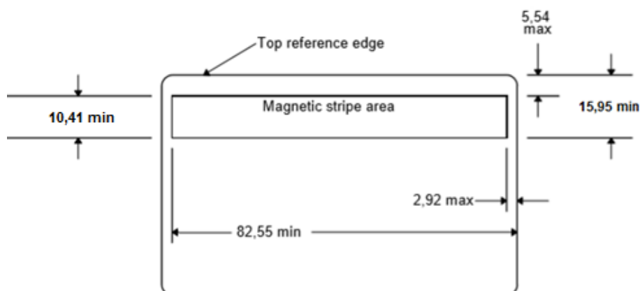
Figure 6 – Magnetic stripe location dimensions (mm)
