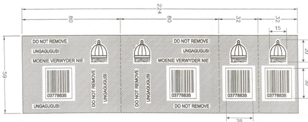
Figure 7 – Meter seal design and dimensions
