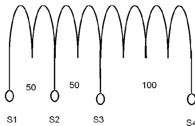
Figure 3: Tapping Arrangements for Multi-ratio 1/200 Measuring Cores
