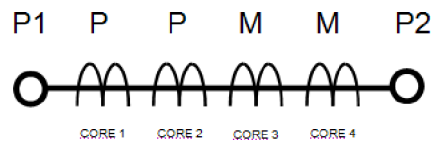
Figure 1: Core Layout – Four-core Current Transformers
