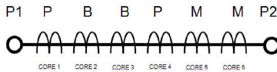
Figure 2: Core Layout – Six-core Current Transformers
