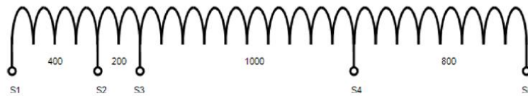
Figure 6: Tapping Arrangements for Multi-ratio 1/2 400t
