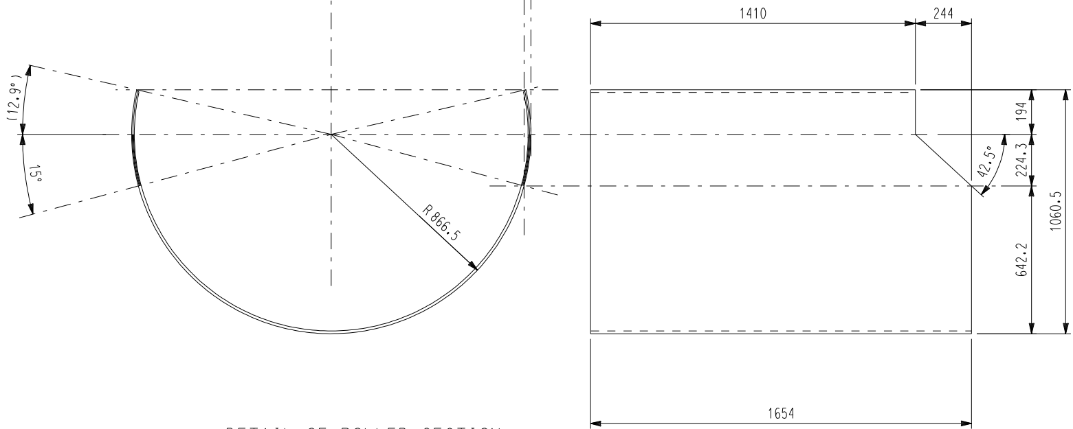
DETAIL OF ROLLED SECTION
