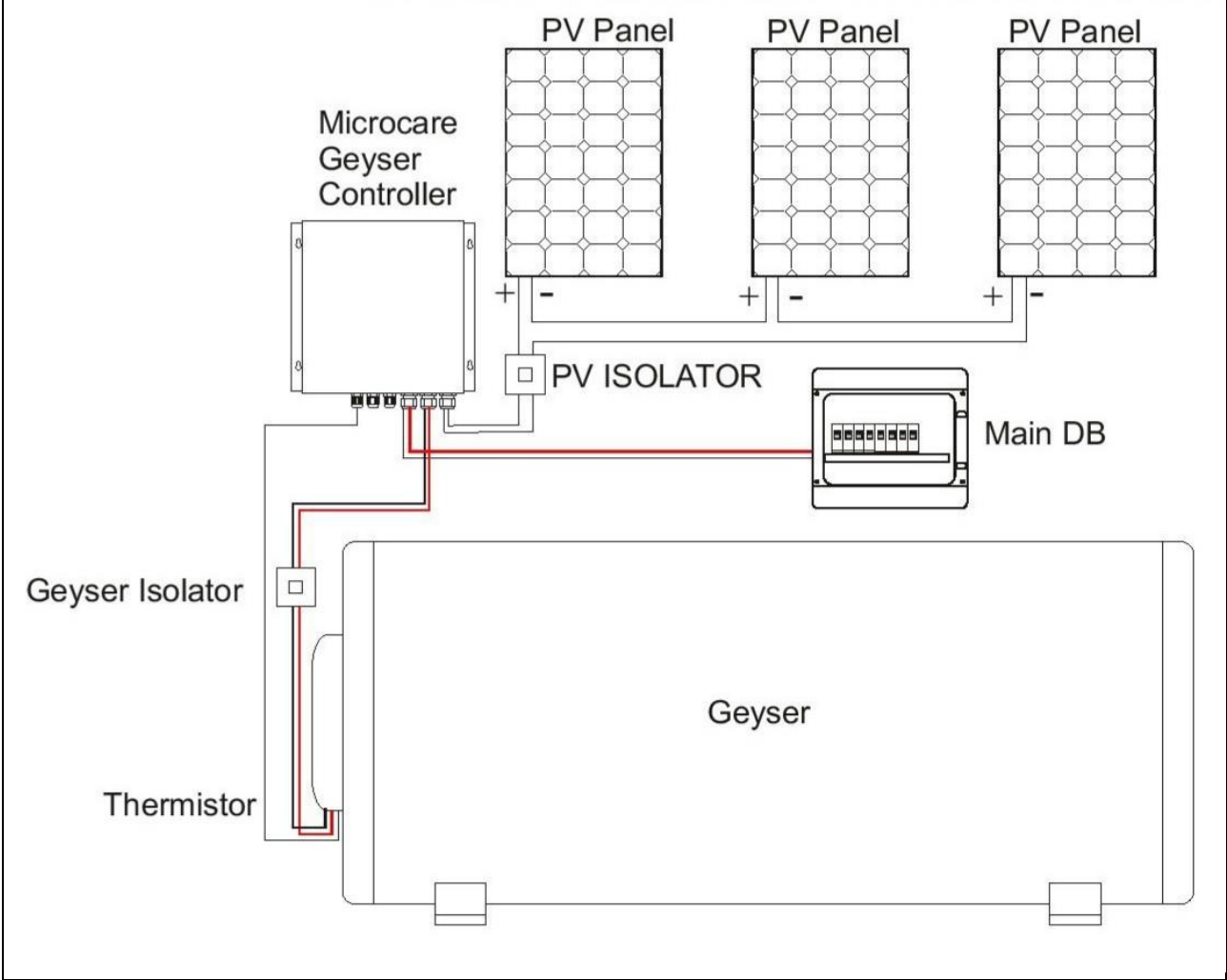
Photo 2: Typical Existing New Solar Geyser (Geysers are moved Outside and Solar panels can be anywhere)
