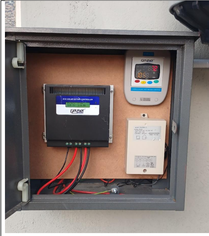
Photo 3: New Existing Solar Geyser Control Panel board
