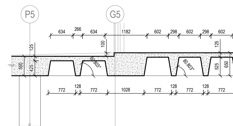
TYPICAL SECTION: COFFER SLAB STEP DOWN SCALE 1:50
