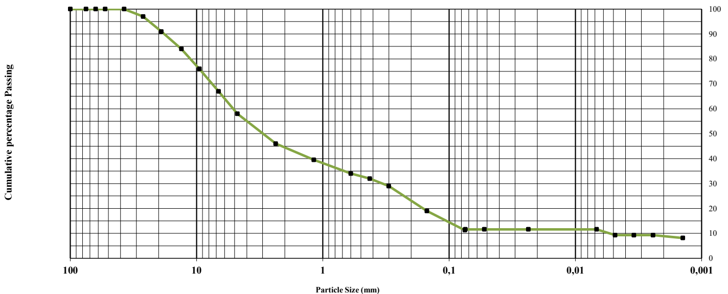
Particle Size Distribution
