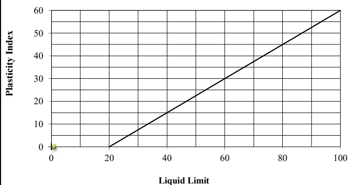
Plasticity Chart A Line
