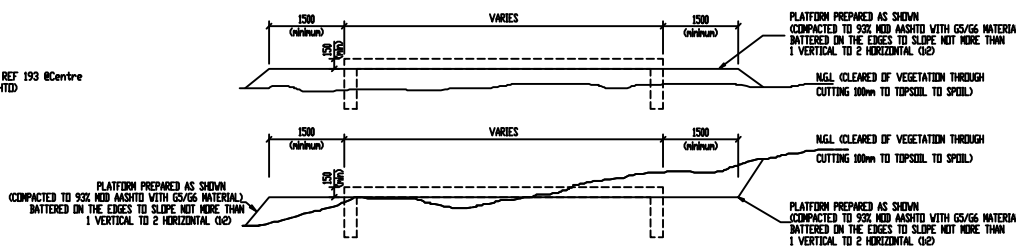
PLATFORM PREPARATIONS DETAILS (FOR STORMWATER CONTROL) (HORIZONTAL 1:50 & VERTICAL 1:25)
