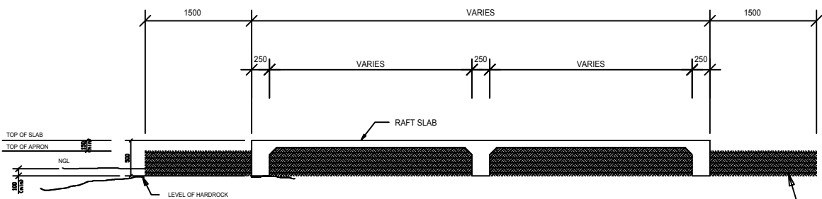
TYPICAL SECTION (PLATFORM ON NEAR SURFACE HARDROCK)
