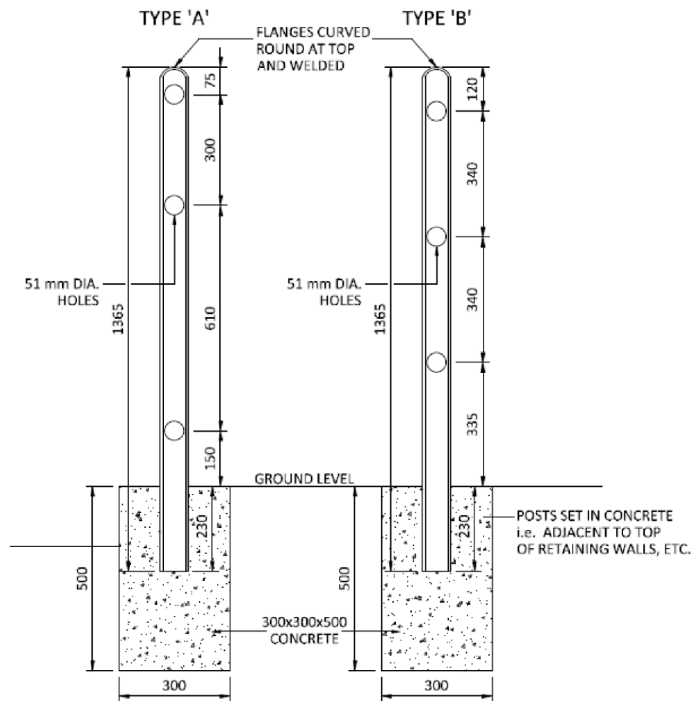
SECTIONS OF CHANNELS
