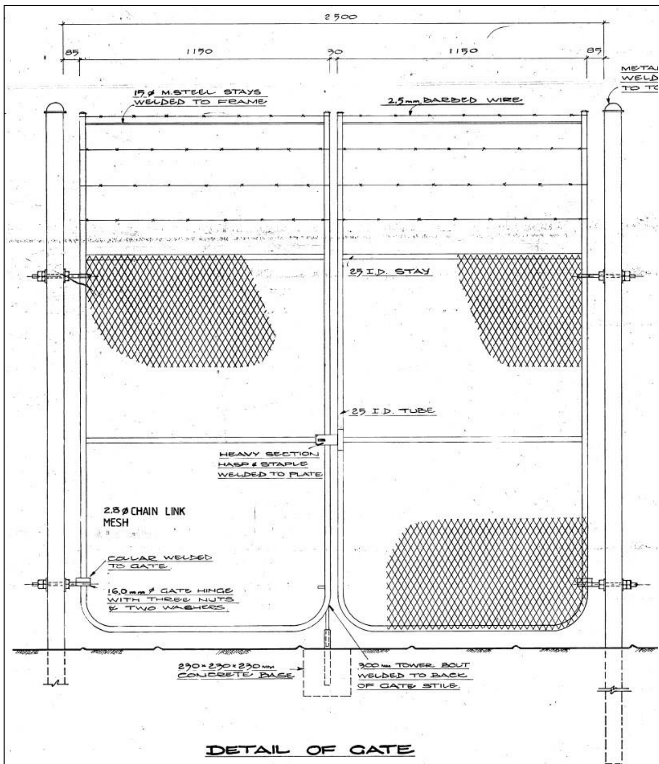
Figure 6. Item 55 (LHS) and 56 (RHS) - Drawing: PRA 2080 Rev 6
