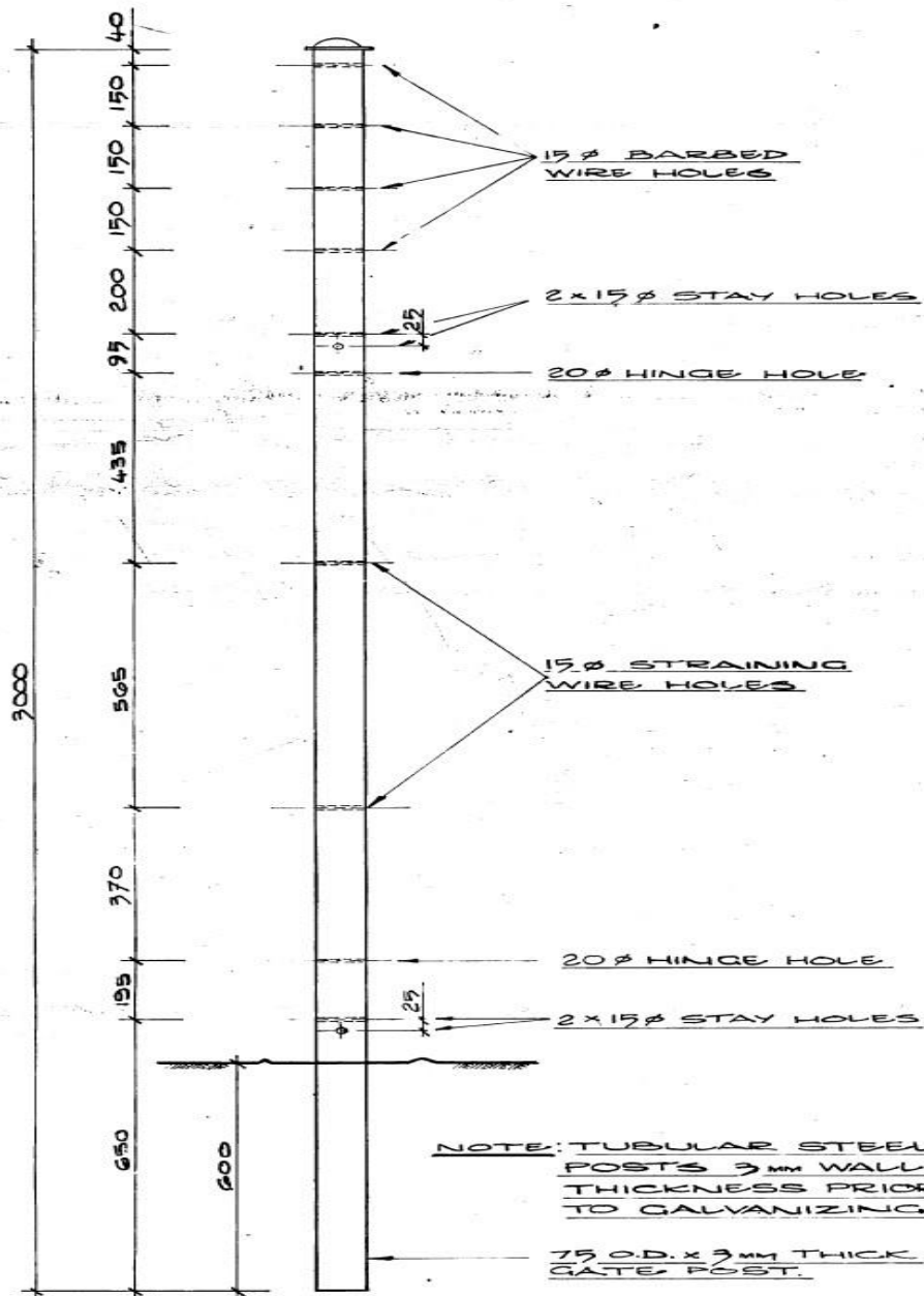
DETAIL OF POST
