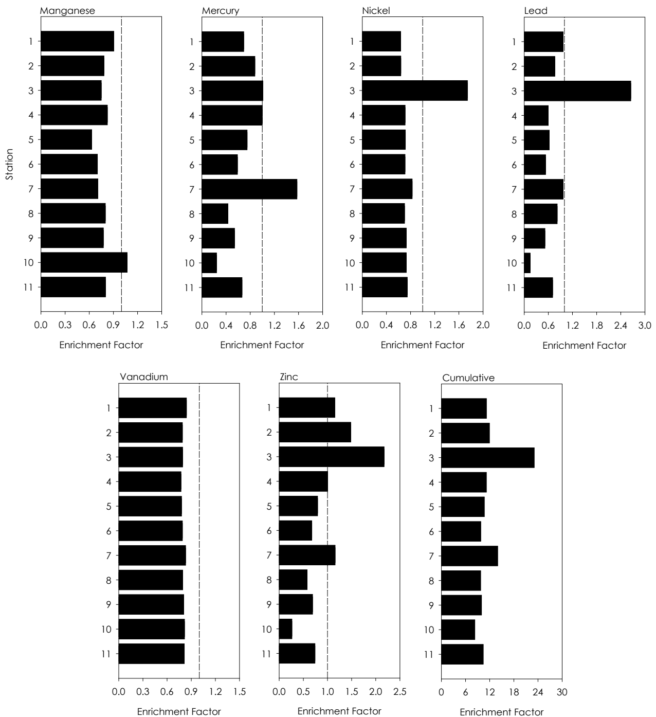
Figure 8 continued. Enrichment Factors for metals in sediment sampled in the Buffalo River estuary in July 2022. The dashed lines represent an Enrichment Factor = 1. An Enrichment Factor >1 indicates the metal was at a concentration exceeding the baseline and may indicate contamination.
