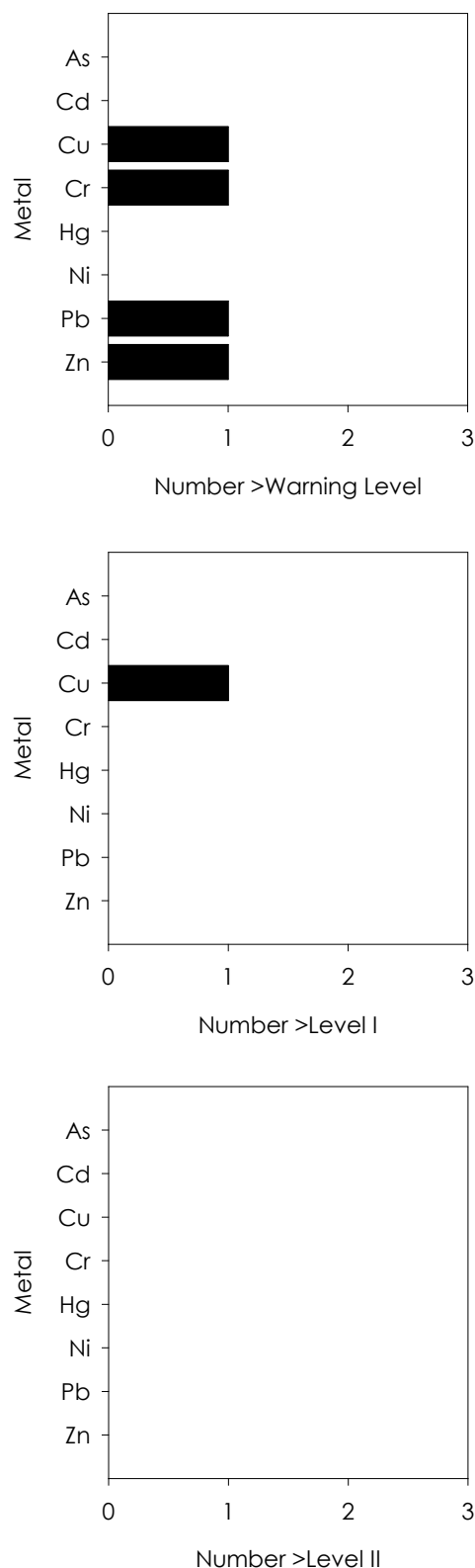
Figure 9. The number of stations at which metals in sediment sampled in the Buffalo River estuary in July 2022 were at a concentration that exceeded the Warning Level, Level I and Level II of the sediment quality guidelines used by the Department of Forestry, Fisheries and the Environment to decide if sediment identified for dredging in South African ports is suitable for open water disposal.
