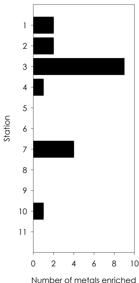
Figure 6. The number of metals enriched in sediment sampled in the Buffalo River estuary in July 2022.
