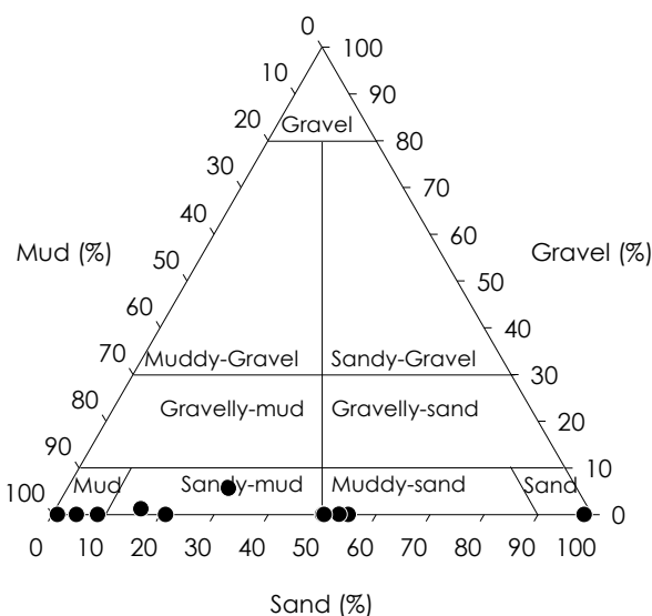
Figure 2. Ternary plot illustrating the proportional contribution of gravel, sand, and mud to the bulk weight of sediment sampled in the Buffalo River estuary in July 2022.
