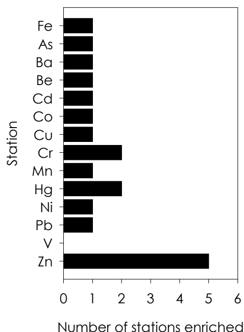
Figure 7. The number of stations in the Buffalo River estuary where sediment sampled in July 2022 was enriched by various metals.
