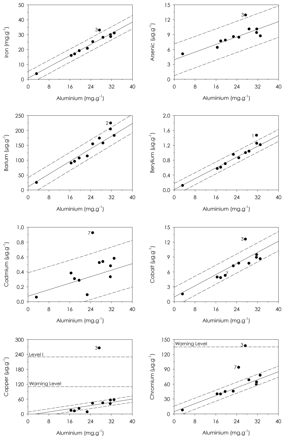
Figure 4. Baseline metal concentration models for sediment in the Buffalo River estuary, with metal concentrations in sediment sampled in the estuary in July 2022 superimposed. Sediment quality guidelines used by the Department of Forestry, Fisheries and the Environment to decide if sediment identified for dredging in South African ports is suitable for open water disposal are included if they fall within the y-axis range. Some metal concentrations are highlighted by station identifiers.
