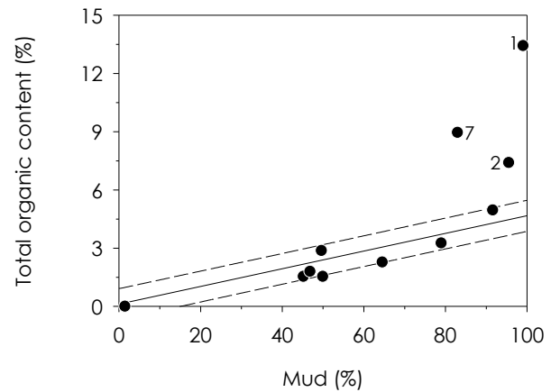
Figure 3. Baseline model for total organic content in sediment in the Buffalo River estuary, with the total organic content in sediment sampled in the estuary in July 2022 superimposed. Some data points are highlighted by station identifiers.
