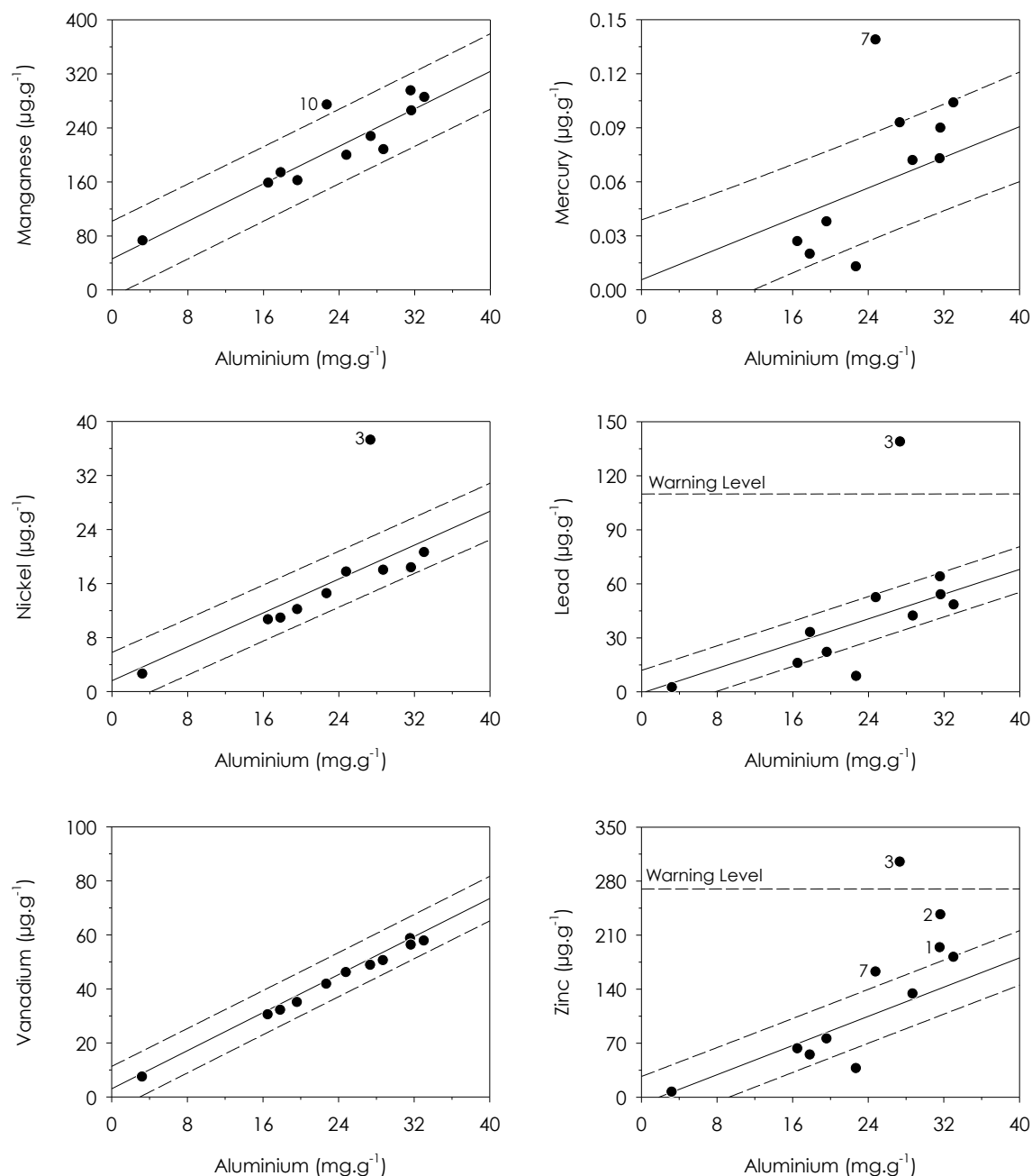
Figure 4 continued. Baseline metal concentration models for sediment in the Buffalo River estuary, with metal concentrations in sediment sampled in the estuary in July 2022 superimposed. Sediment quality guidelines used by the Department of Forestry, Fisheries and the Environment to decide if sediment identified for dredging in South African ports is suitable for open water disposal are included if they fall within the y-axis range. Some metal concentrations are highlighted by station identifiers.
