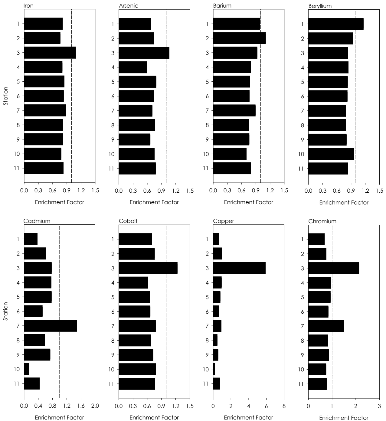
Figure 8. Enrichment Factors for metals in sediment sampled in the Buffalo River estuary in July 2022. The dashed lines represent an Enrichment Factor = 1. An Enrichment Factor >1 indicates the metal was at a concentration exceeding the baseline and may indicate contamination.
