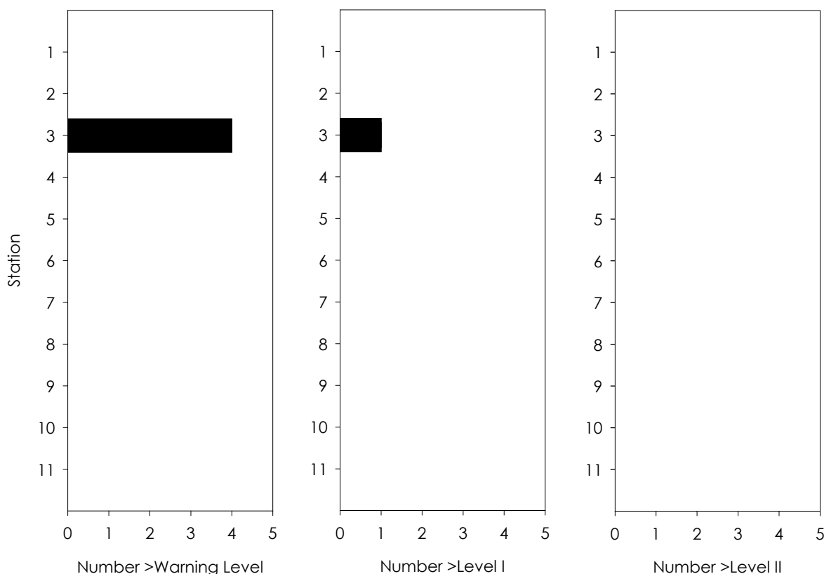
Figure 10. The number of stations at which metals in sediment sampled in the Buffalo River estuary in July 2022 were at a concentration that exceeded the Warning Level, Level I and Level II of the sediment quality guidelines used by the Department of Forestry, Fisheries and the Environment to decide if sediment identified for dredging in South African ports is suitable for open water disposal.
