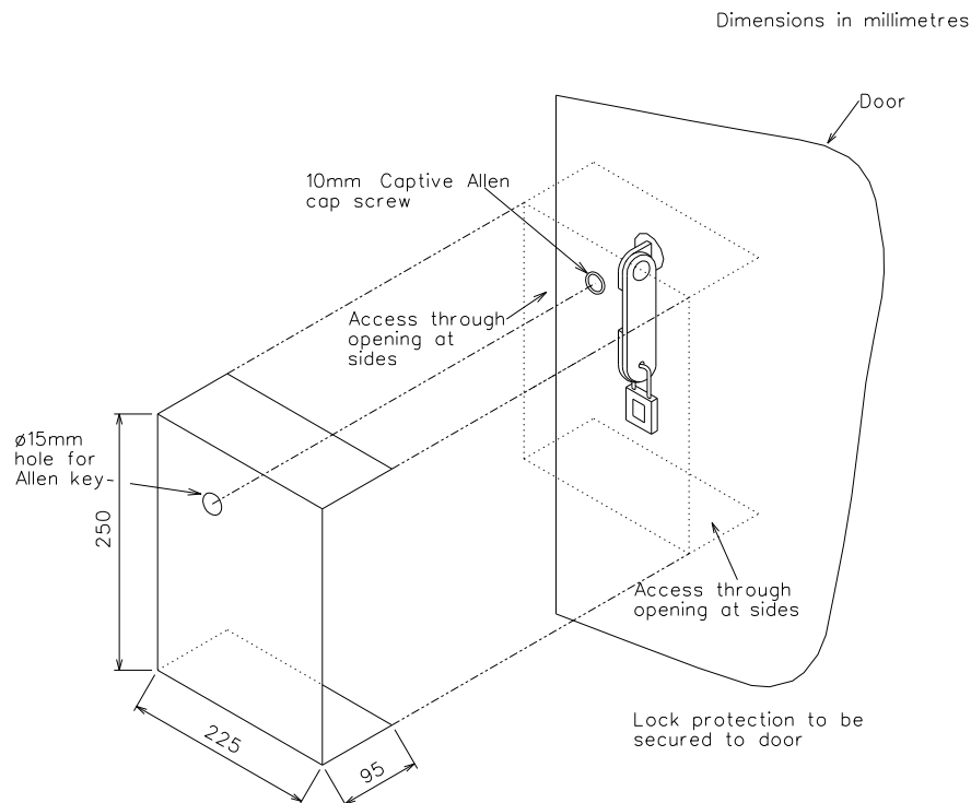
Figure 1: Outdoor kiosk padlock protection facility
