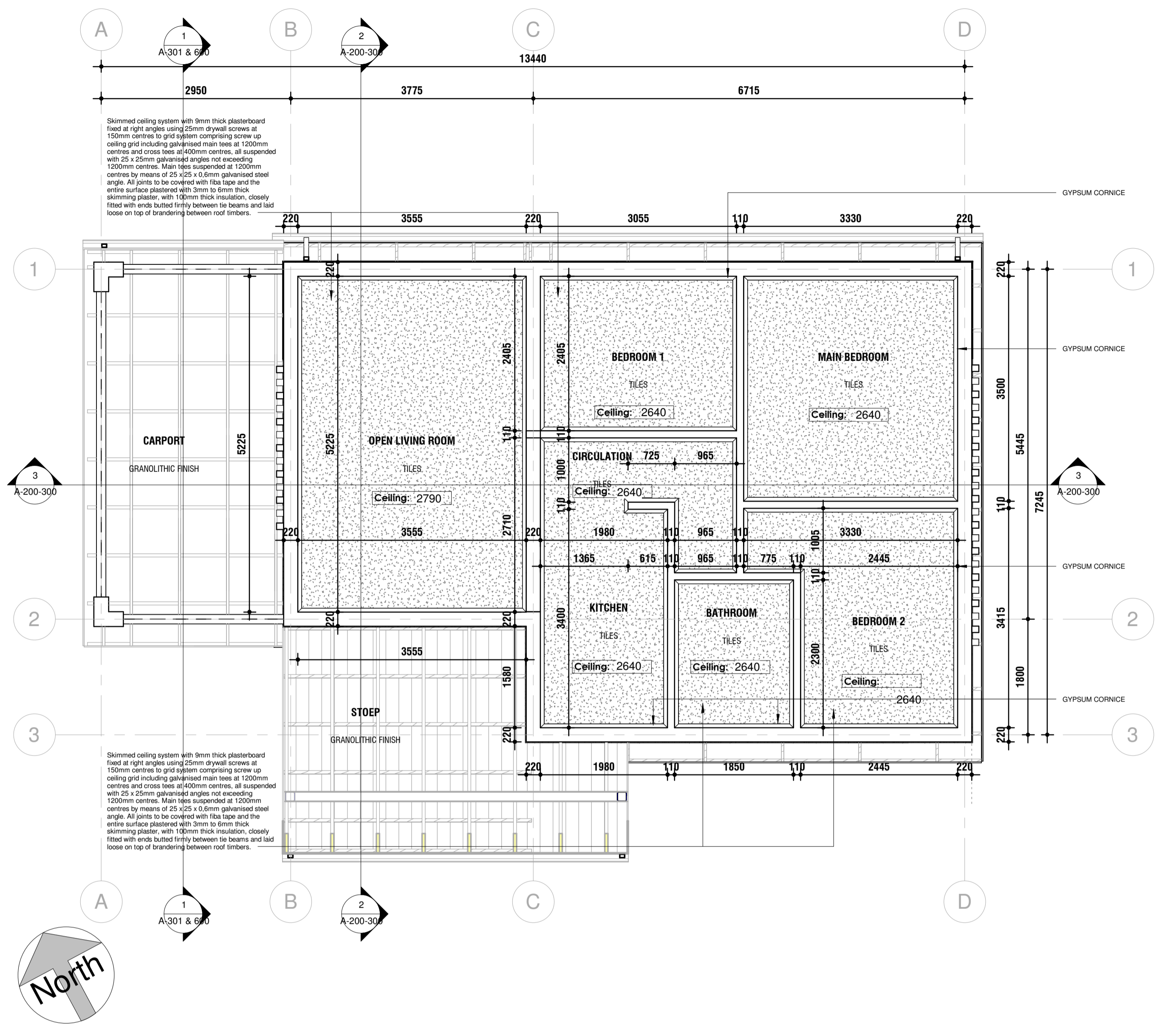
1 Ground Floor Ceiling Plan 1 : 50
