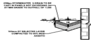
V-DRAIN DETAIL ALONG WALL SECTION SCALE 1:20
