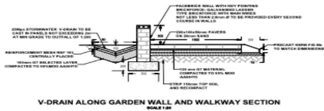
V-DRAIN ALONG GARDEN WALL AND WALKWAY SECTION SCALE 1:30
