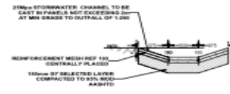
TRAPEZOIDAL CHANNEL DETAIL SCALE 1:20
