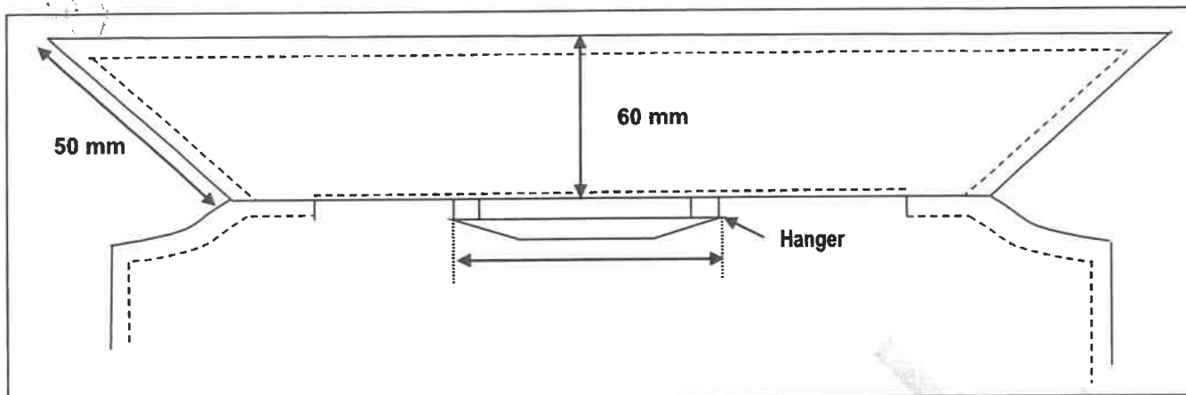
Figure 10 – Collar
