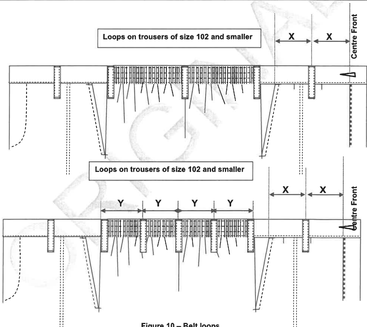
Figure 10 – Belt loops
