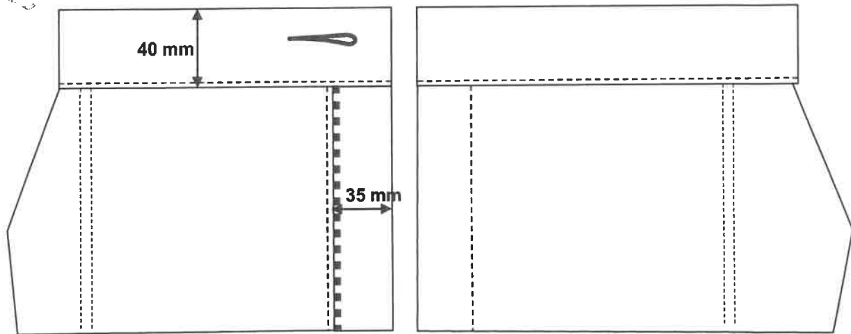
Figure 5 – Fly-catch
