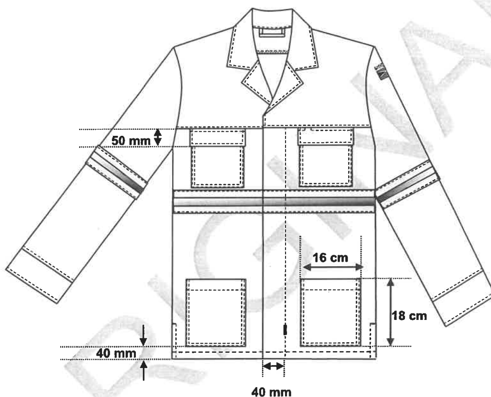
Figure 7 – Pocket positioning
