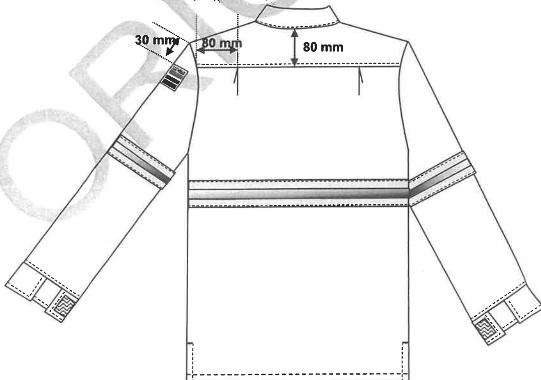
Figure 9 – Back view
