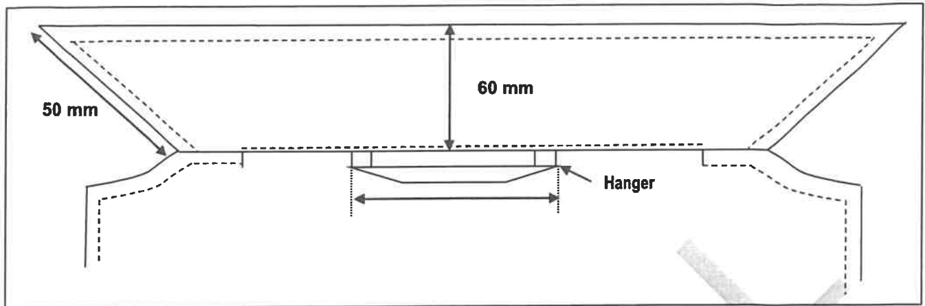
Figure 8 – Collar
