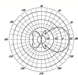
Y460-7 Vertical
