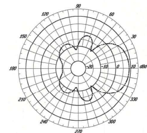
Y460-7 Horizontal
