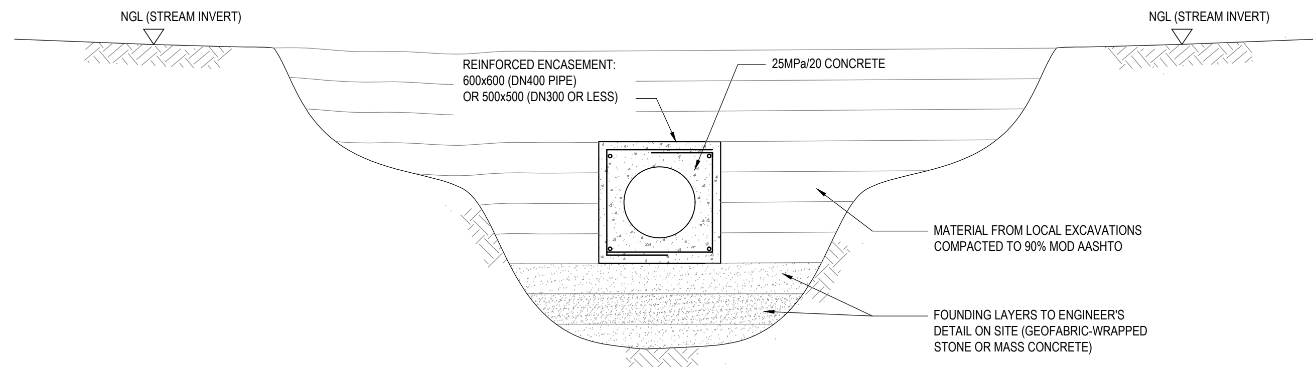
TYPICAL SECTION ENCASEMENT IN SOFT MATERIAL
