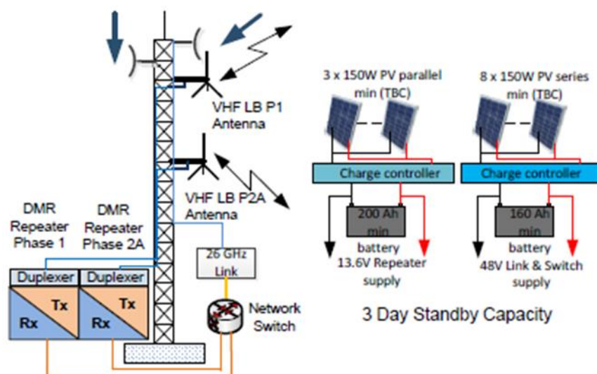
Figure 2: DMR high site infrastructure
