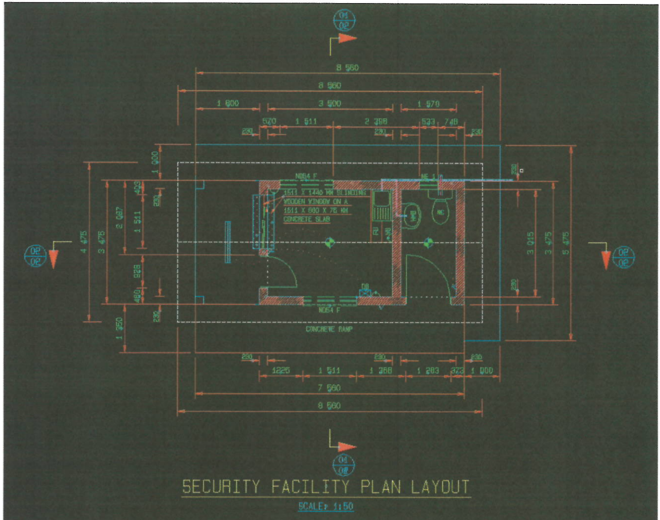
Picture 1: showing a dimensioned type drawing plan layout of a security facility brick building.
