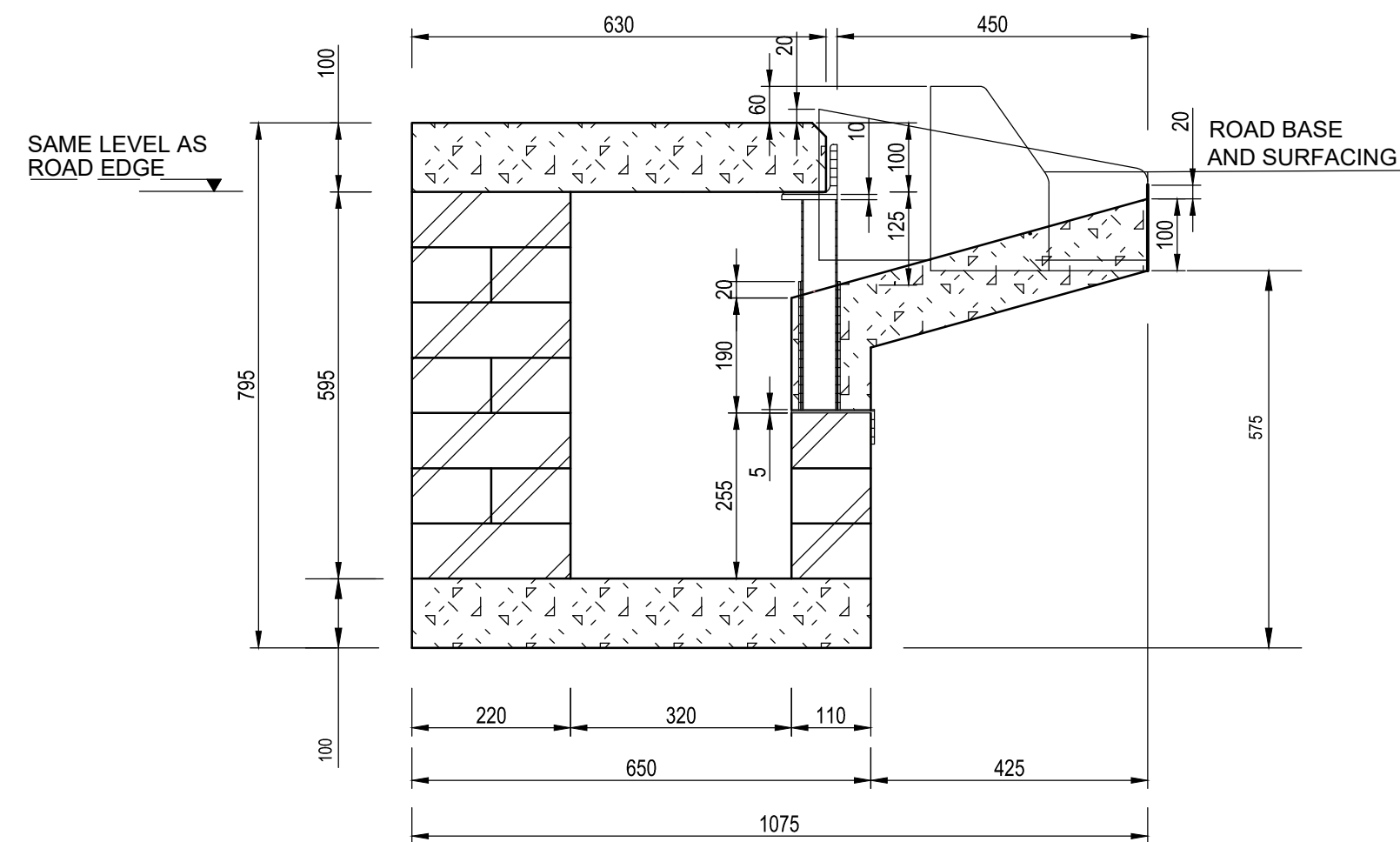
SECTION C-C SCALE 1:10
