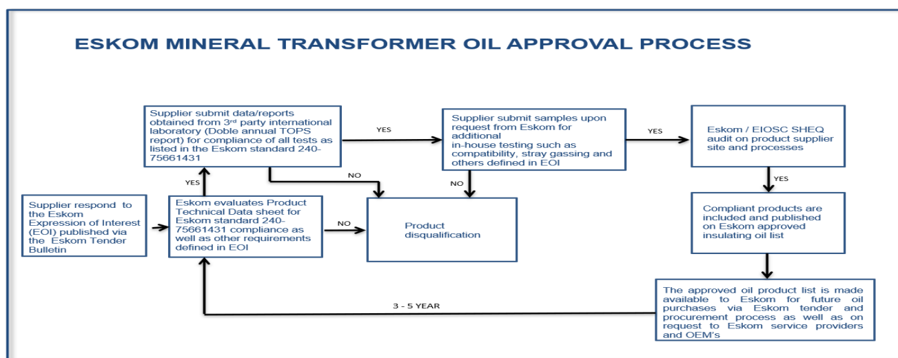
Figure 1: Mineral transformer oil process for compilation of Eskom approved oil list
