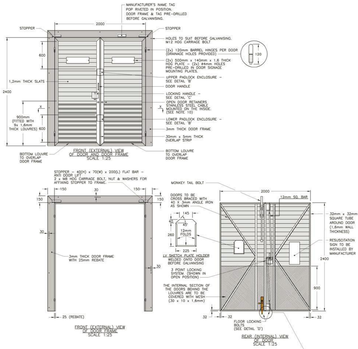
Drawing No. 3 Double Door (1600mm x 2400mm)
