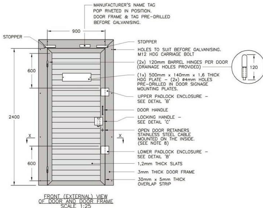
Drawing No. 1 Single Door (900mm x 2400mm)
