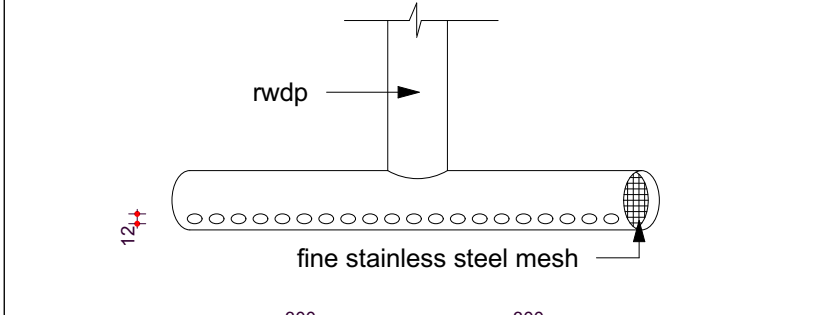
Detail 100-04 - SPREADER DETAIL Scale 1:10
