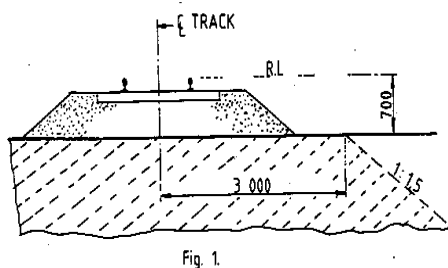
Formation level
