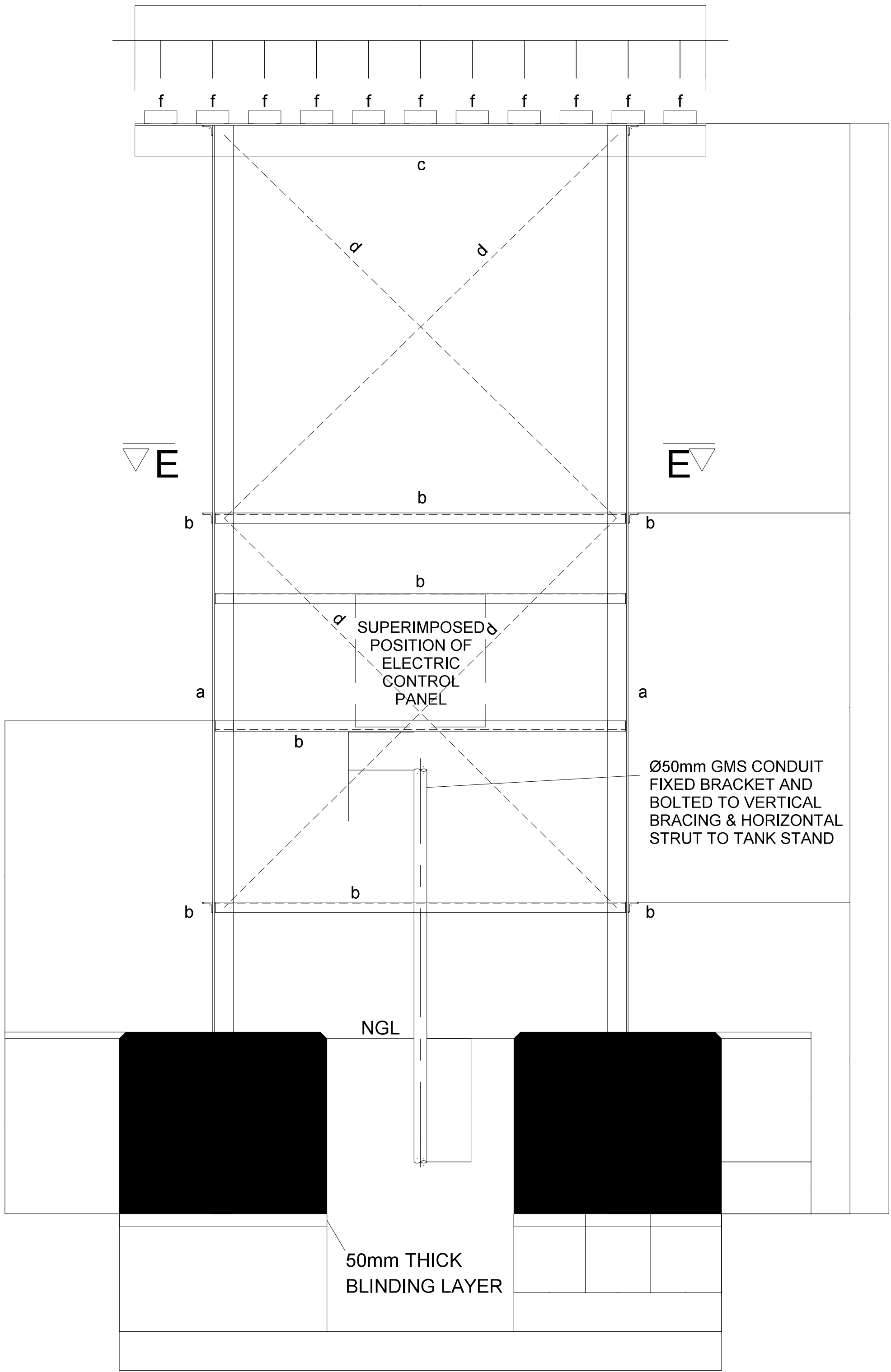
SECTION C-C
