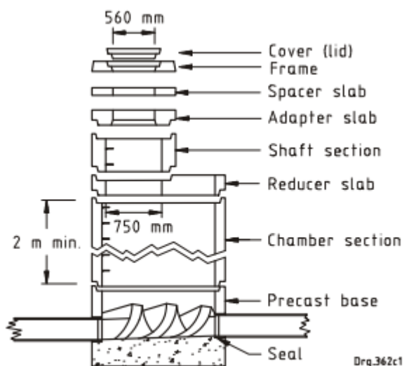
Figure 2(a) — Composition of a manhole
