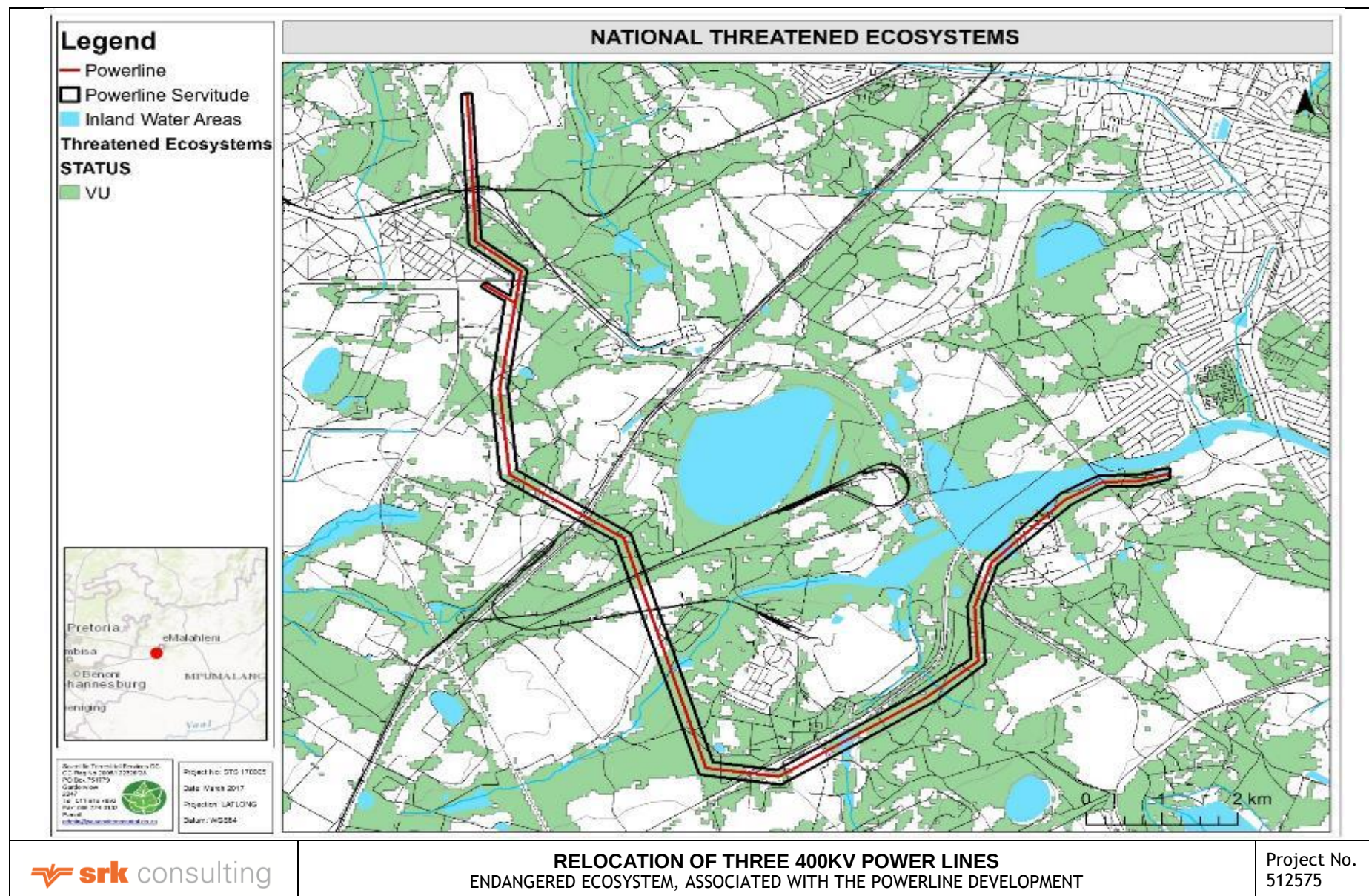
Figure 5-10: Endangered ecosystem, associated with the power line development according to the National Threatened Ecosystem Database (2011)
