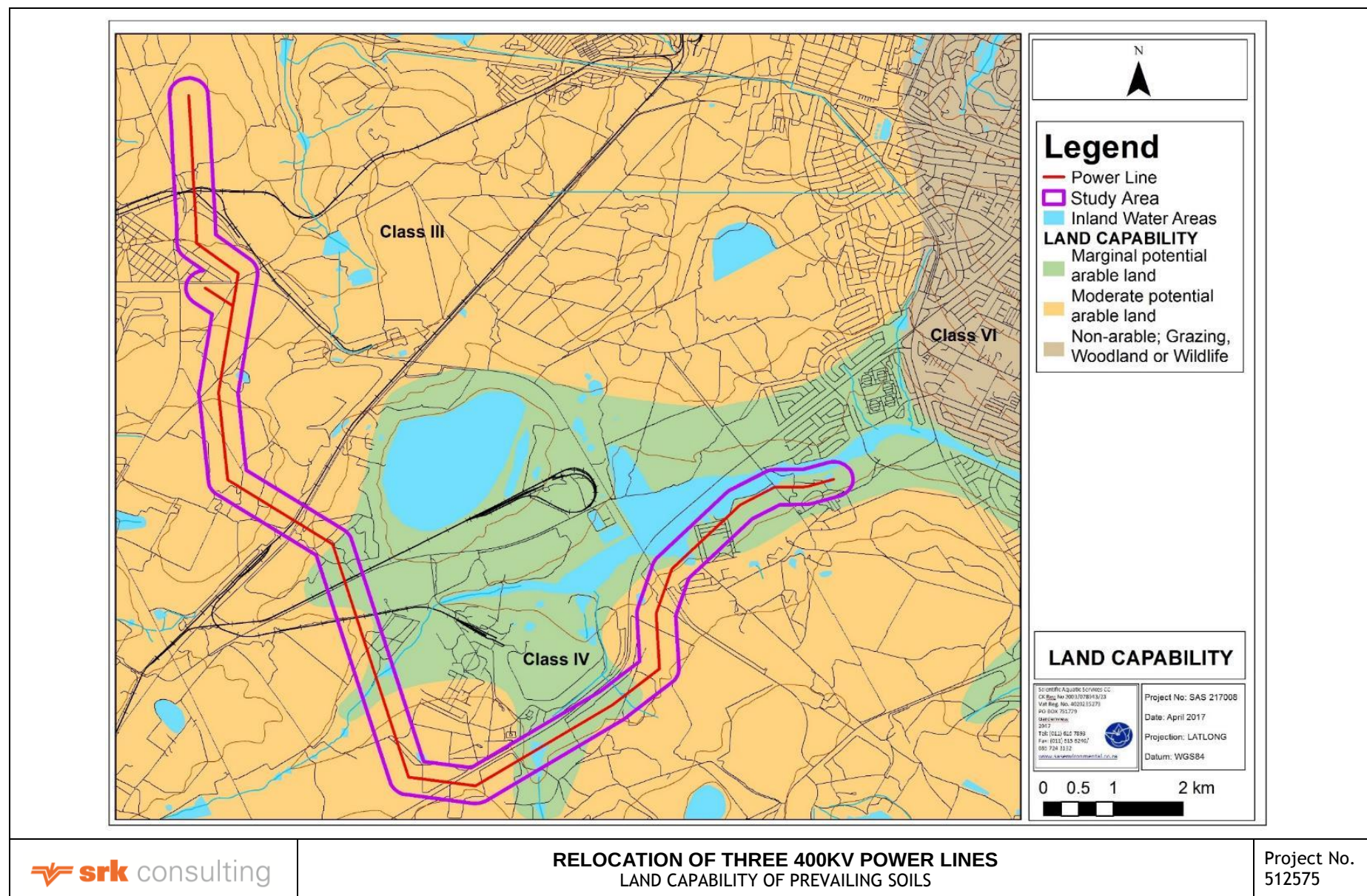
Figure 5-5: Land capability of the prevailing soils in the vicinity of the study area according to the AGIS database
