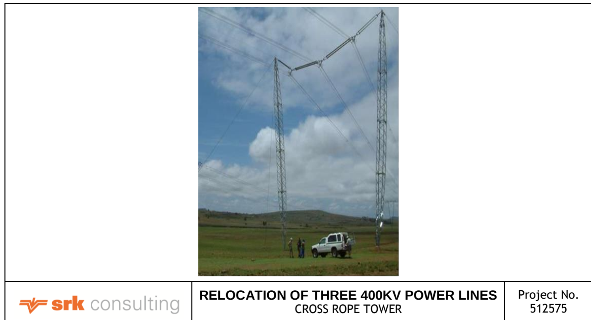
Figure 4-8: Cross rope tower
