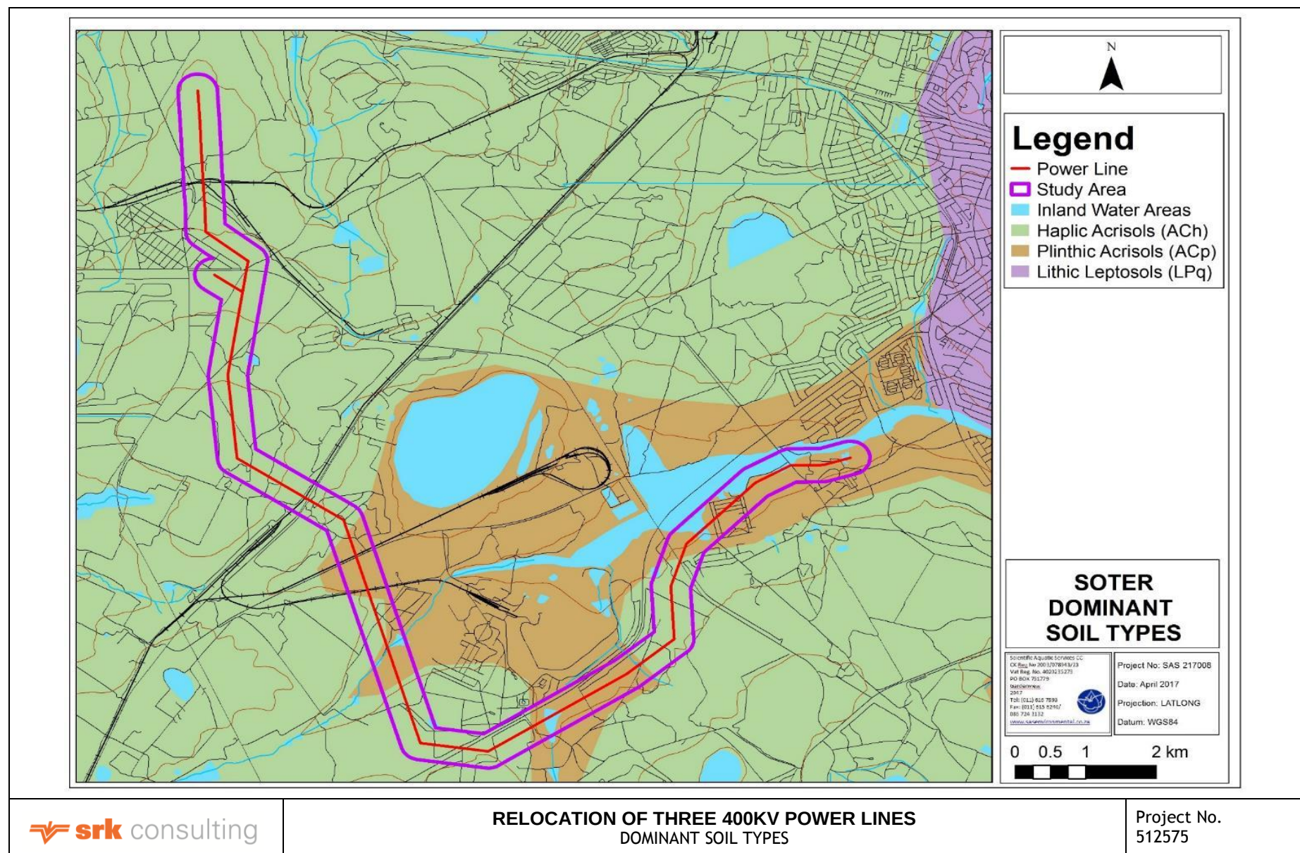
Figure 5-4: Dominant soil types in the vicinity of the study area according to the SOTER database.
