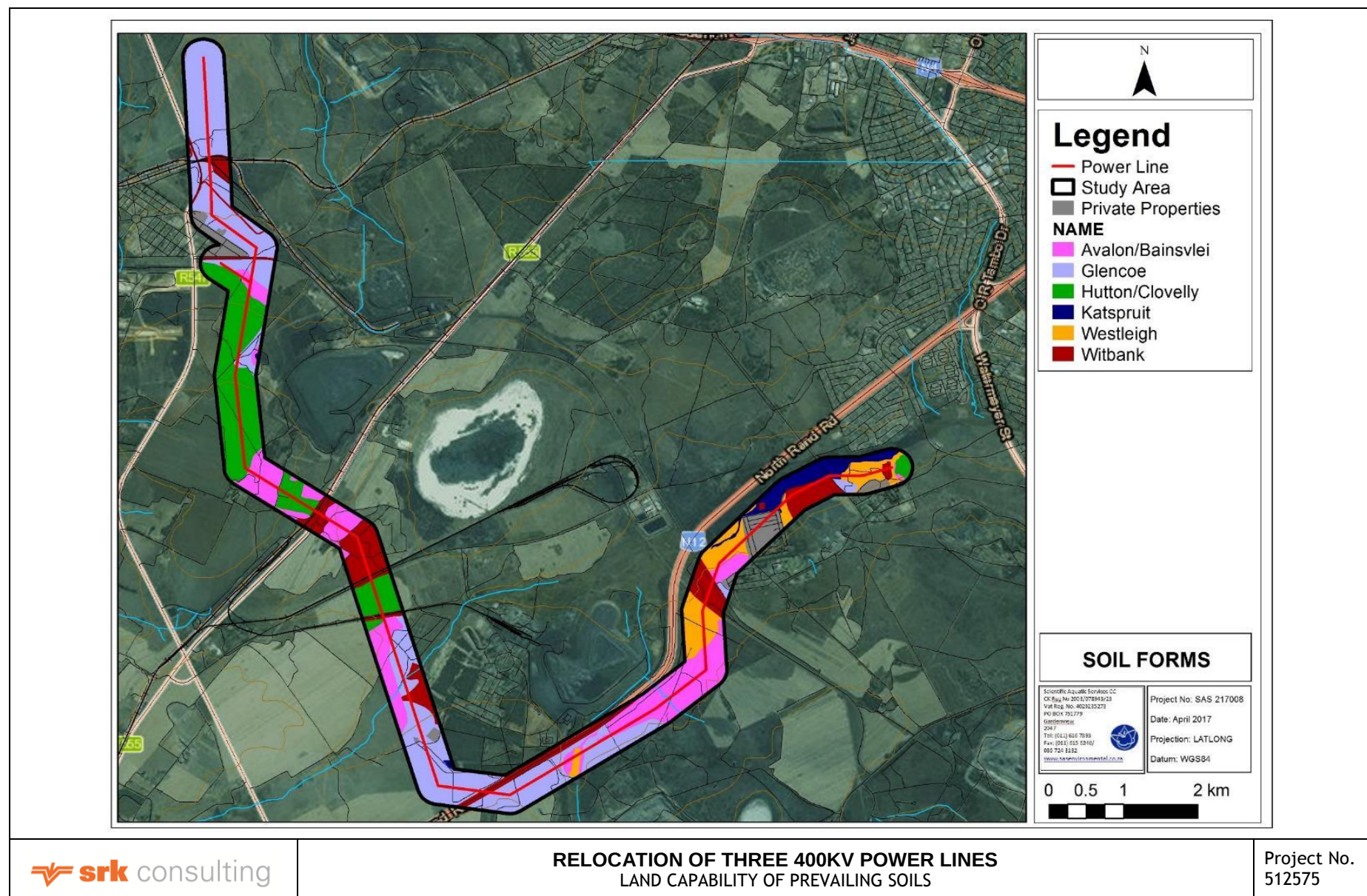
Figure 5-7: Soil map depicting identified soil forms within the study area
