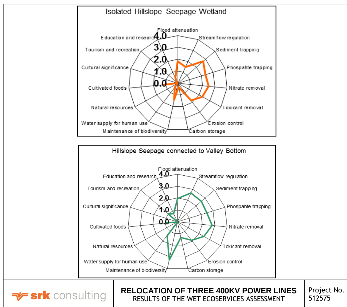
Figure 5-37: Radial plots showing the results of the WET-EcoServices assessment.
