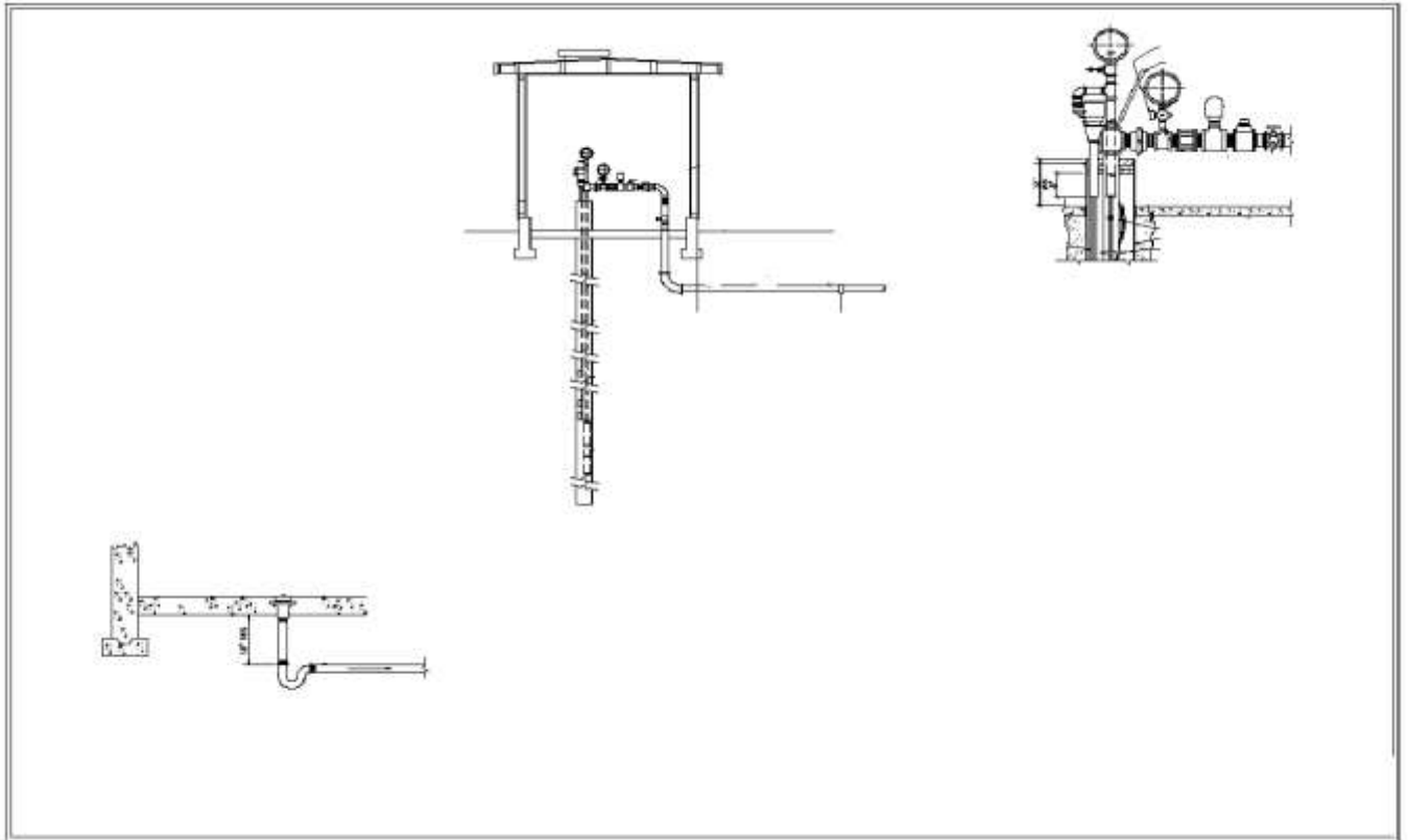
Borehole pump installation with pump safety : Pump safety detail as per standard Borehole pump installation:
