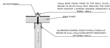
INTERNAL PARTITION WALL TO ROOF FIXING DETAIL
