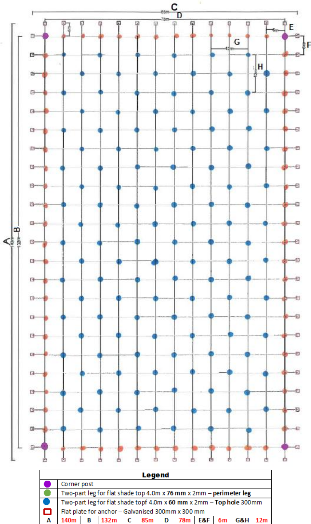
Figure 4 Positioning of poles
