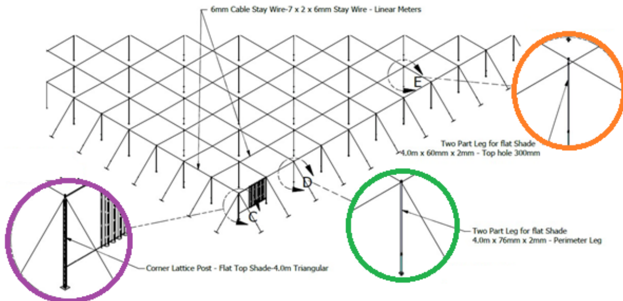
Figure 5 Detail of different poles
