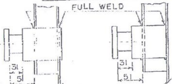
DETAIL 'A'
