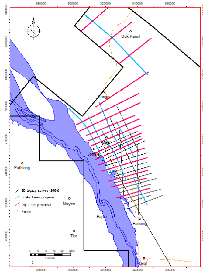
Figure #3: Tentative 2D Seismic layout map
