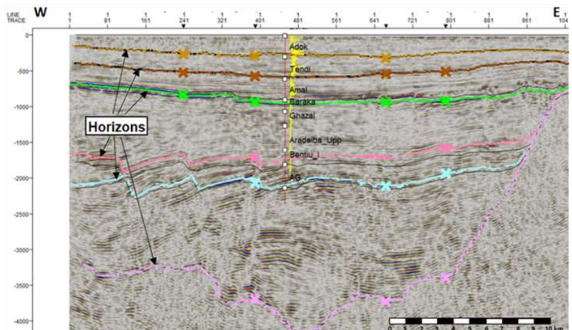
Figure #4: Existing SEG Y 2D line (black in figure #1) oriented W_E direction. The seismic section is intercepted by the well Kedelai-1 and shows the interpretation of key geological horizon
