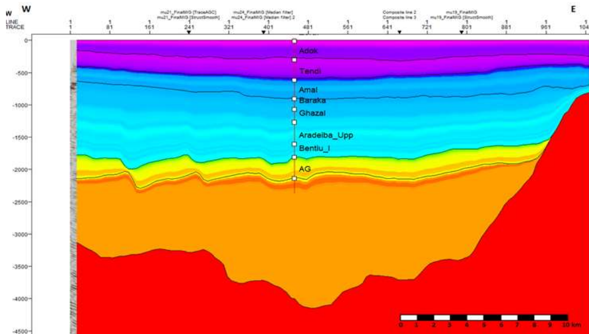
Figure # 5: Interval velocity section (black line in figure #1) generated using velocity data from wells in vicinity field.
