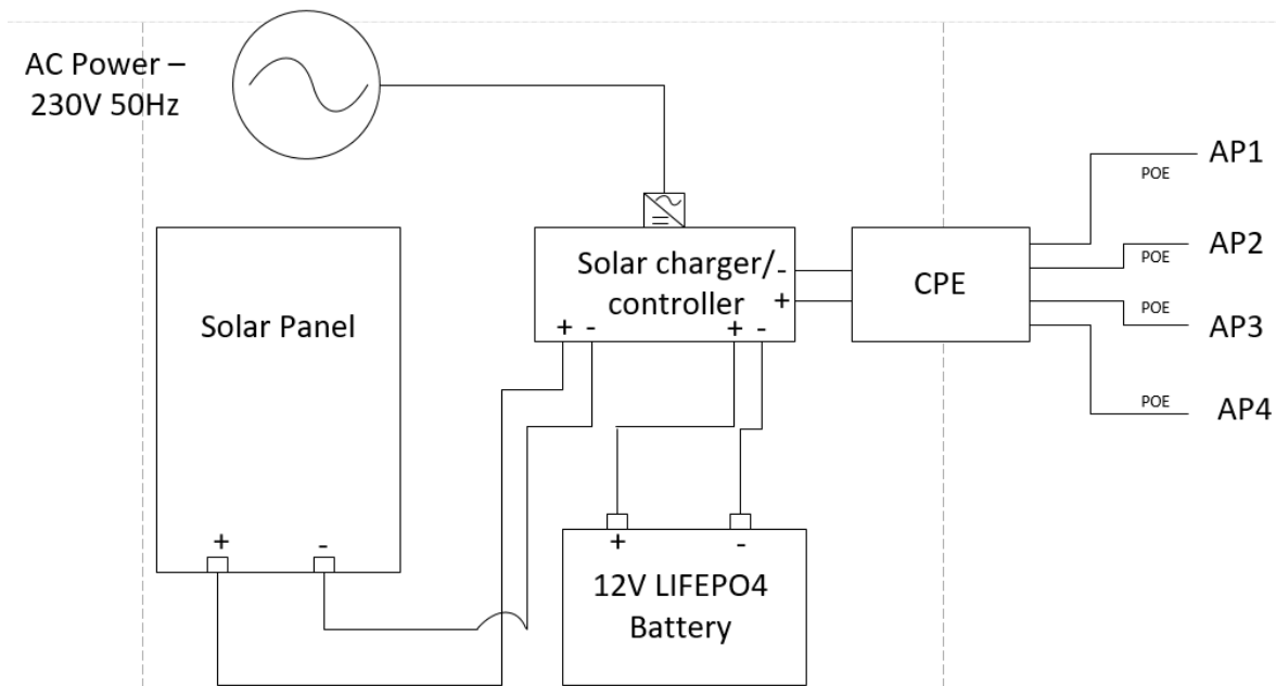
UPS solution with typical components and connections
