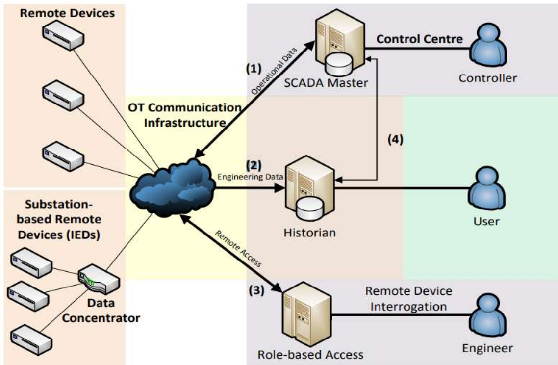
Figure 1: Data Acquisition Architecture
