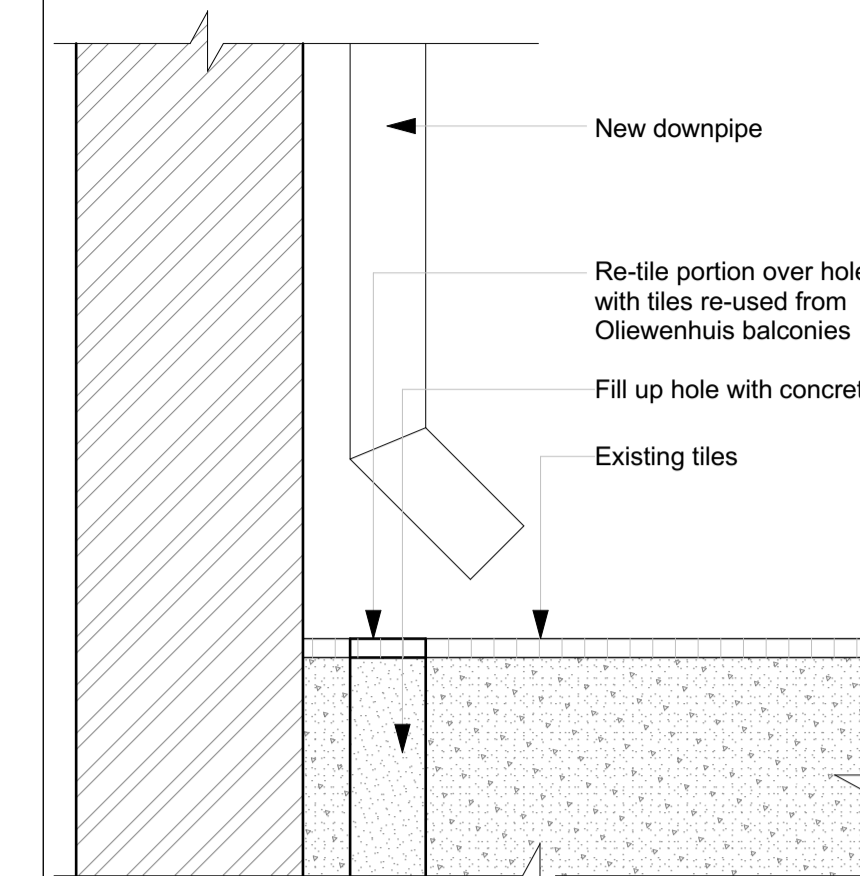
Detail 100-02 - DOWNPIPE DETAIL Scale 1:10
